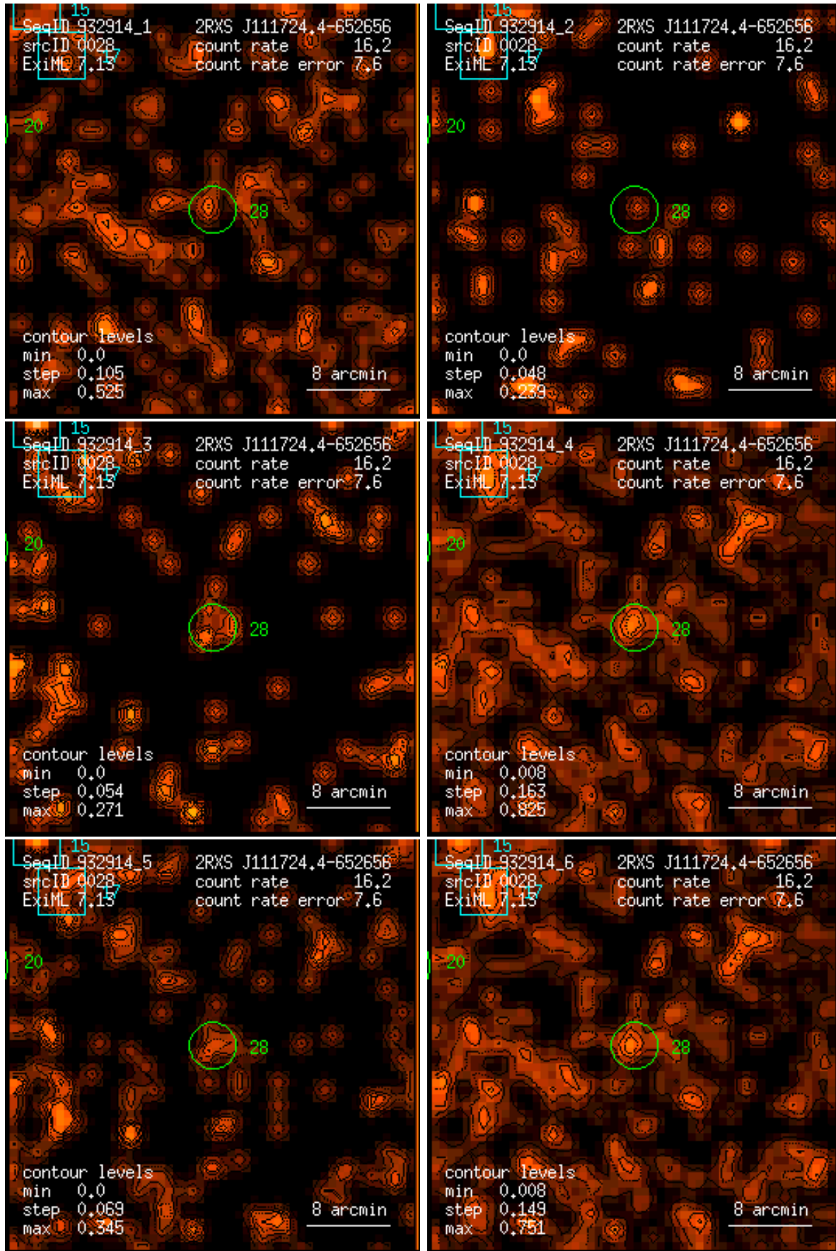
Figure 28: RASS 932914: detection 0028: band rate images, Gaussian filter: (1) PSPC channels 11 – 41, (2) 52 – 90, (3) 91 – 201, (4) 11 – 235, (5) 52 – 201, (6) 11 – 201. Broad band rates in counts/ks. Band rate contour levels in counts/ks/arcmin 2 .
