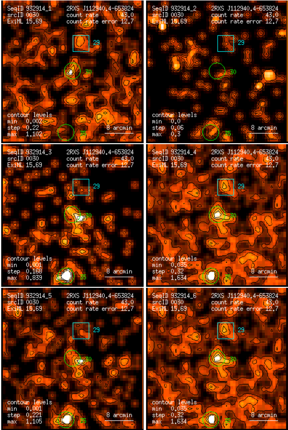
Figure 30: RASS 932914: detection 0030: band rate images, Gaussian filter: (1) PSPC channels 11 – 41, (2) 52 – 90, (3) 91 – 201, (4) 11 – 235, (5) 52 – 201, (6) 11 – 201. Broad band rates in counts/ks. Band rate contour levels in counts/ks/arcmin 2 .
