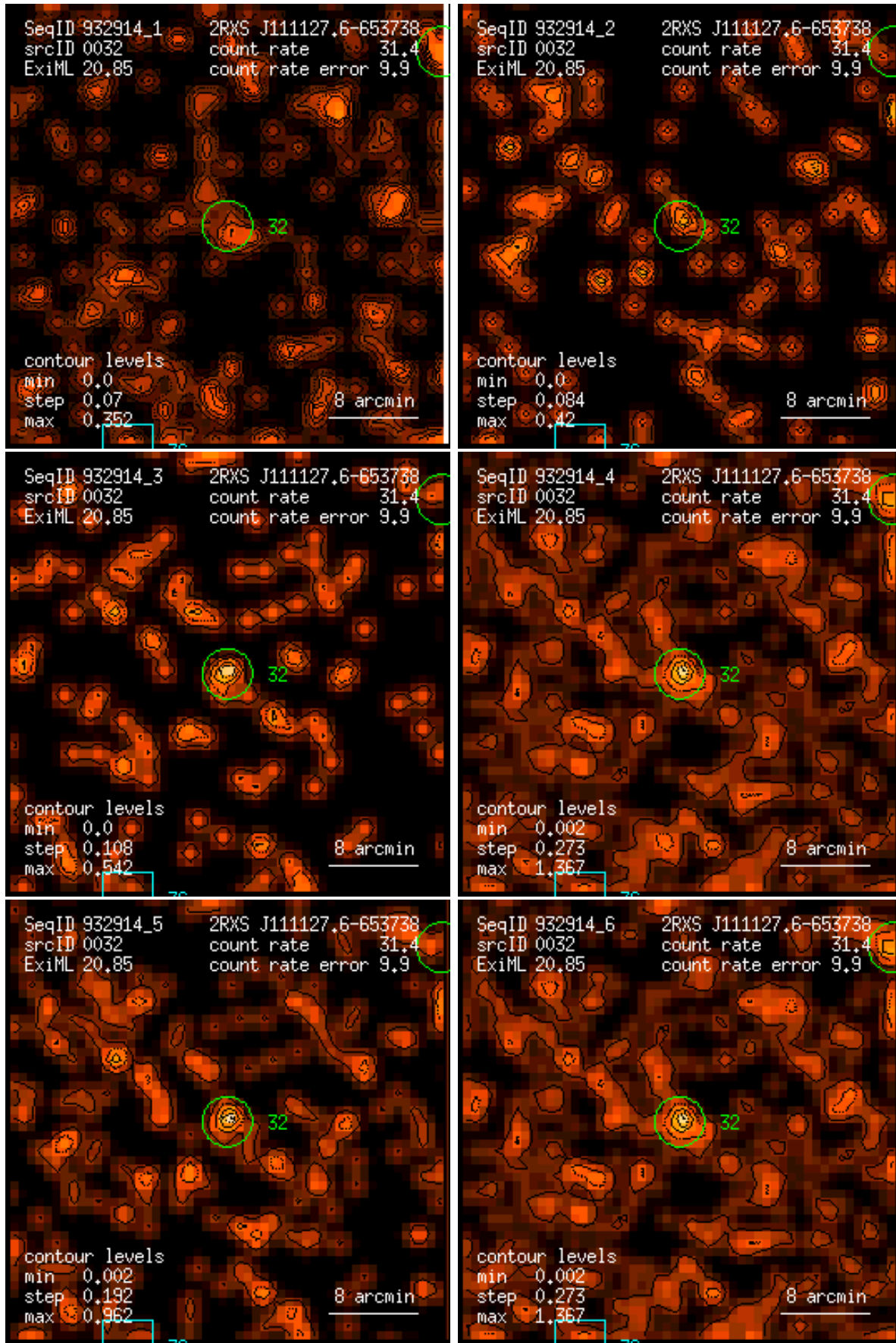
Figure 32: RASS 932914: detection 0032: band rate images, Gaussian filter: (1) PSPC channels 11 – 41, (2) 52 – 90, (3) 91 – 201, (4) 11 – 235, (5) 52 – 201, (6) 11 – 201. Broad band rates in counts/ks. Band rate contour levels in counts/ks/arcmin 2 .
