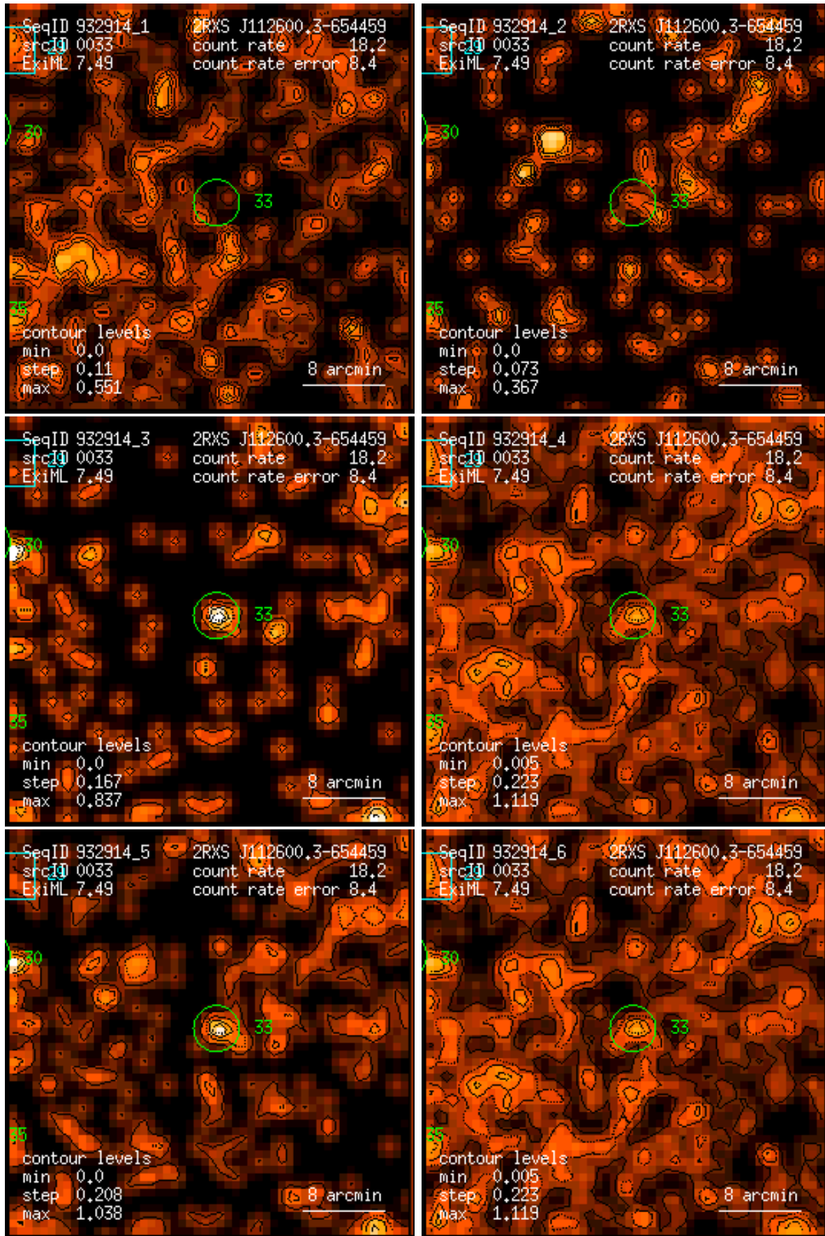
Figure 33: RASS 932914: detection 0033: band rate images, Gaussian filter: (1) PSPC channels 11 – 41, (2) 52 – 90, (3) 91 – 201, (4) 11 – 235, (5) 52 – 201, (6) 11 – 201. Broad band rates in counts/ks. Band rate contour levels in counts/ks/arcmin 2 .
