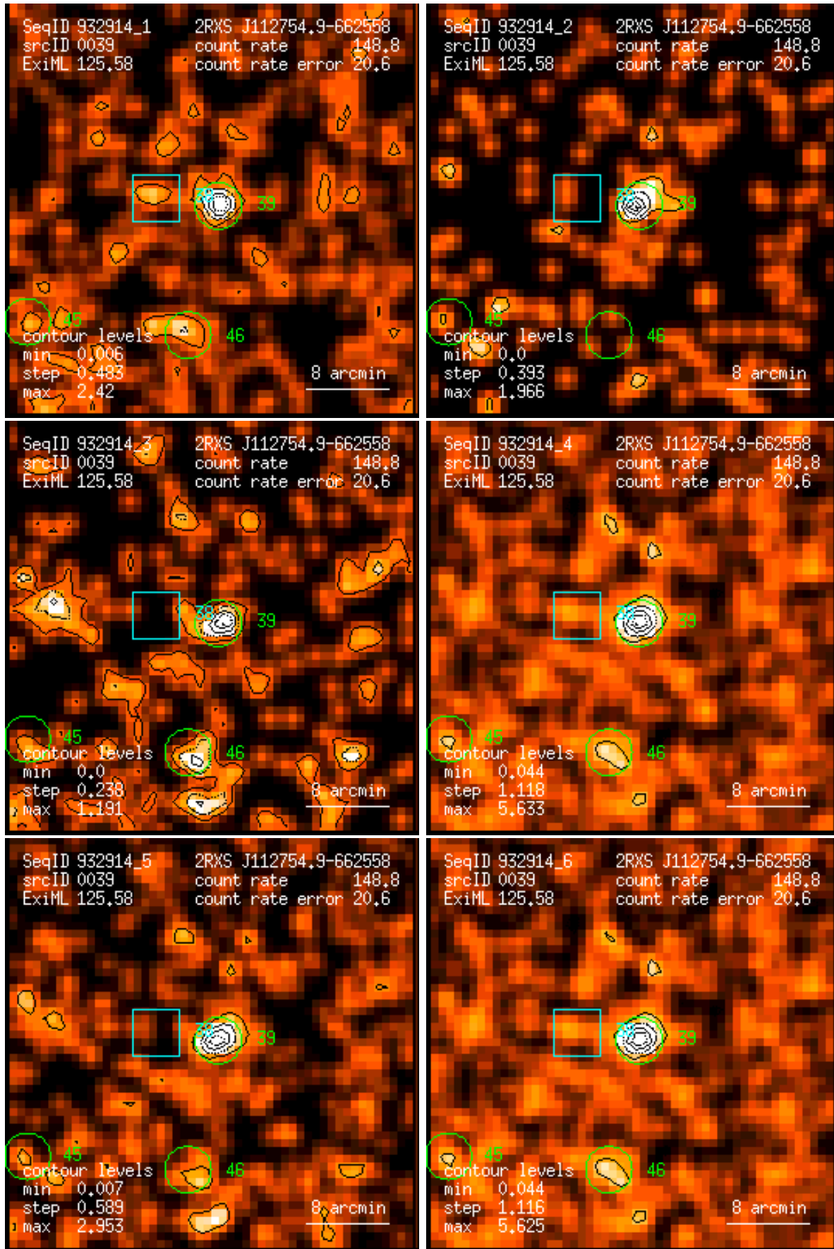
Figure 39: RASS 932914: detection 0039: band rate images, Gaussian filter: (1) PSPC channels 11 – 41, (2) 52 – 90, (3) 91 – 201, (4) 11 – 235, (5) 52 – 201, (6) 11 – 201. Broad band rates in counts/ks. Band rate contour levels in counts/ks/arcmin 2 .
