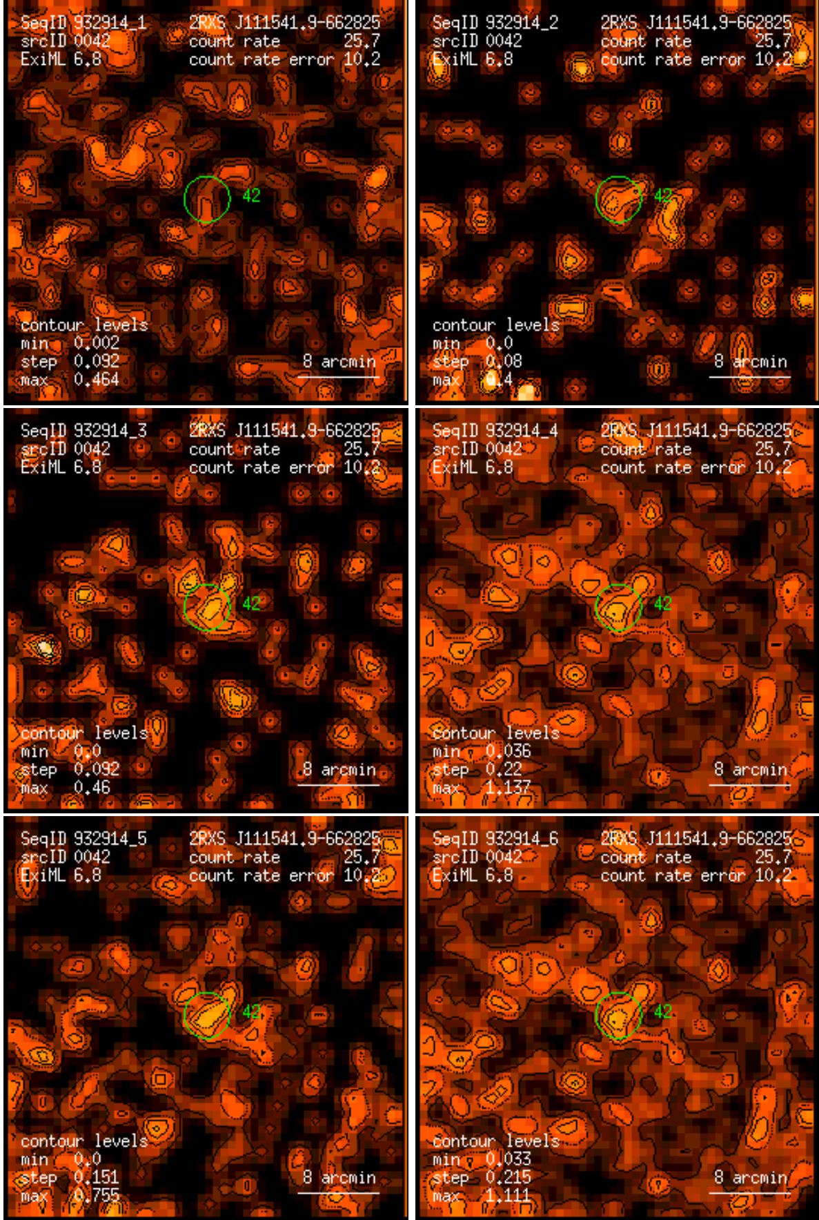
Figure 42: RASS 932914: detection 0042: band rate images, Gaussian filter: (1) PSPC channels 11 – 41, (2) 52 – 90, (3) 91 – 201, (4) 11 – 235, (5) 52 – 201, (6) 11 – 201. Broad band rates in counts/ks. Band rate contour levels in counts/ks/arcmin 2 .
