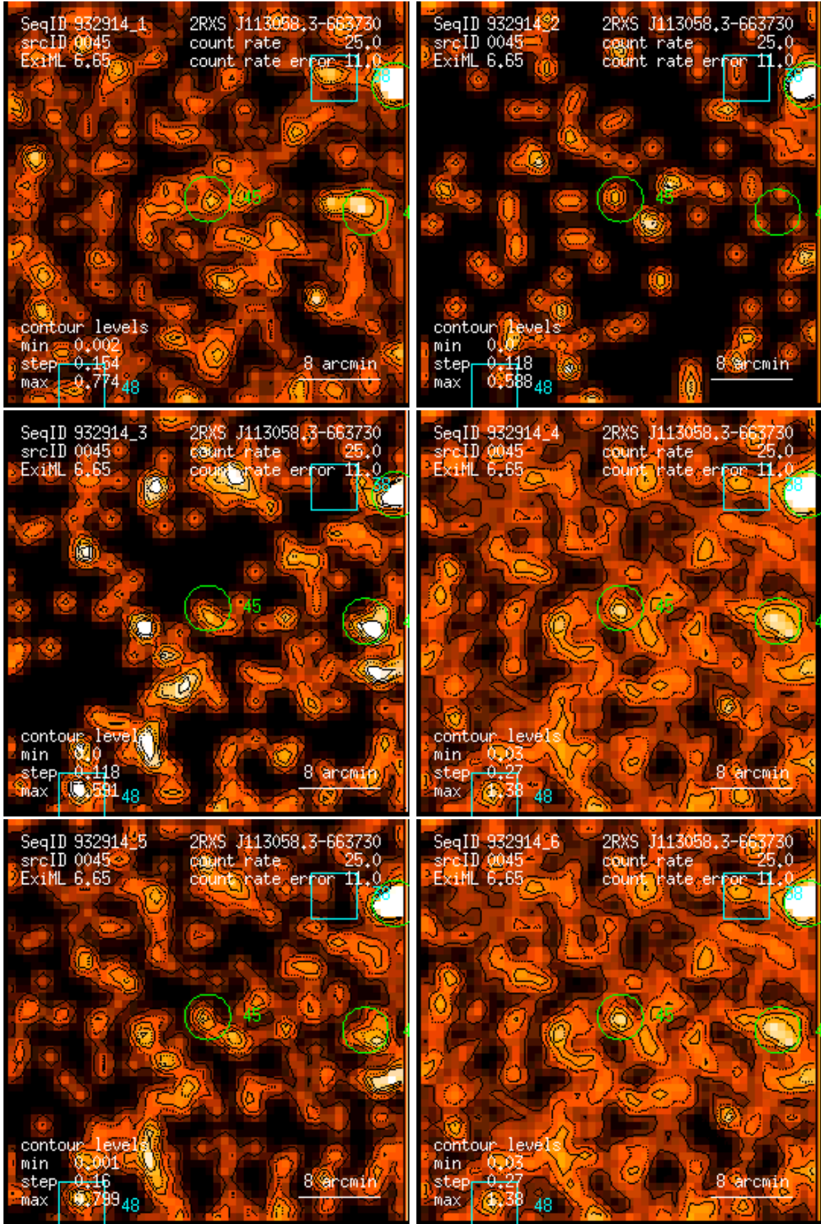
Figure 45: RASS 932914: detection 0045: band rate images, Gaussian filter: (1) PSPC channels 11 – 41, (2) 52 – 90, (3) 91 – 201, (4) 11 – 235, (5) 52 – 201, (6) 11 – 201. Broad band rates in counts/ks. Band rate contour levels in counts/ks/arcmin 2 .
