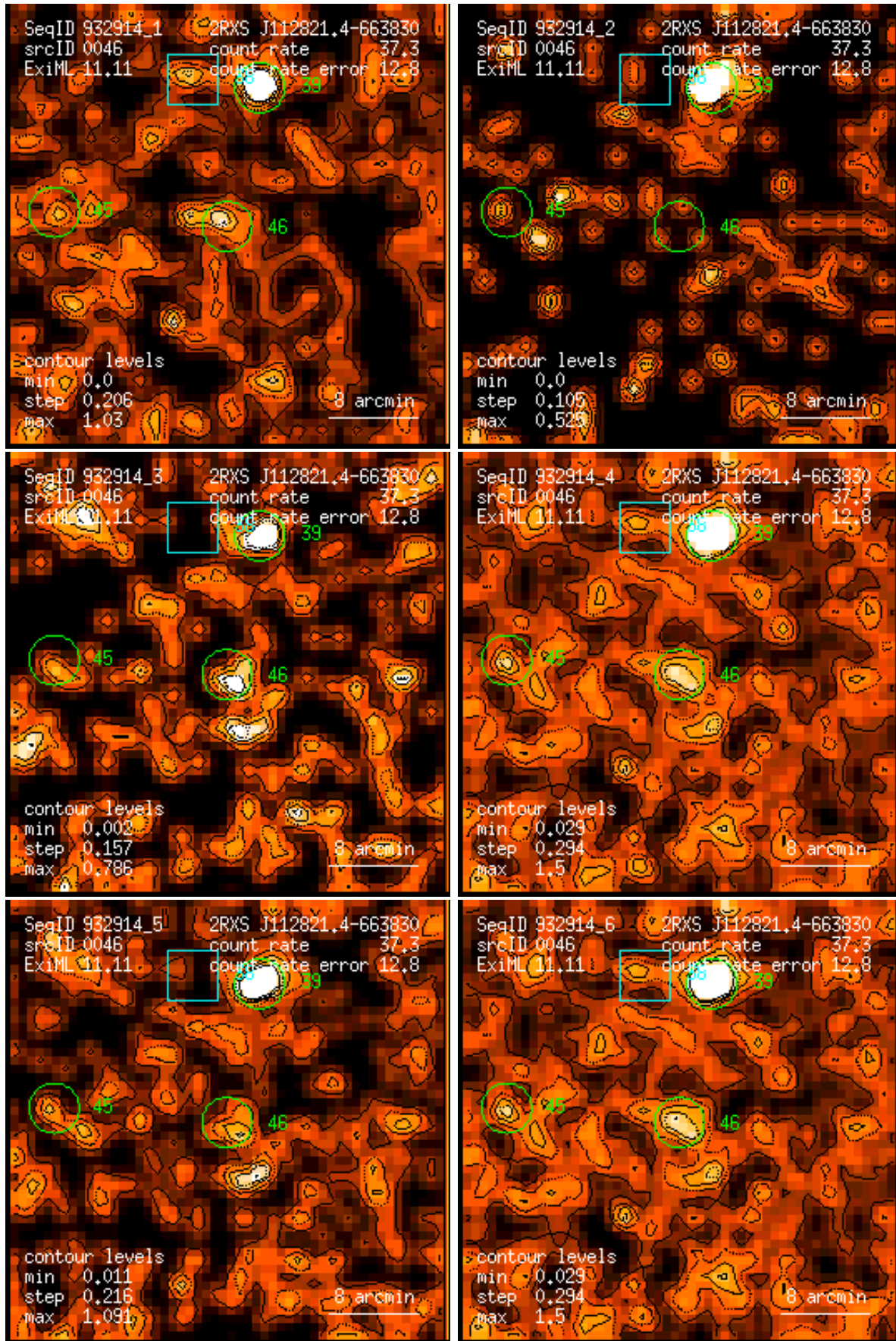
Figure 46: RASS 932914: detection 0046: band rate images, Gaussian filter: (1) PSPC channels 11 – 41, (2) 52 – 90, (3) 91 – 201, (4) 11 – 235, (5) 52 – 201, (6) 11 – 201. Broad band rates in counts/ks. Band rate contour levels in counts/ks/arcmin 2 .
