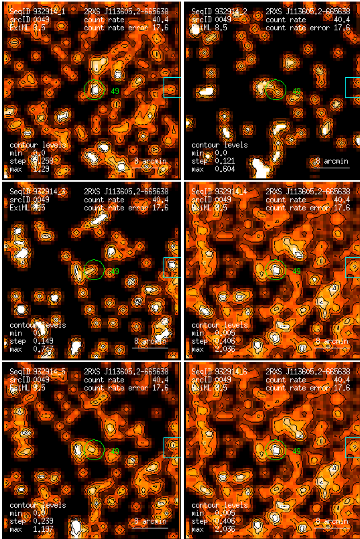
Figure 49: RASS 932914: detection 0049: band rate images, Gaussian filter: (1) PSPC channels 11 – 41, (2) 52 – 90, (3) 91 – 201, (4) 11 – 235, (5) 52 – 201, (6) 11 – 201. Broad band rates in counts/ks. Band rate contour levels in counts/ks/arcmin 2 .
