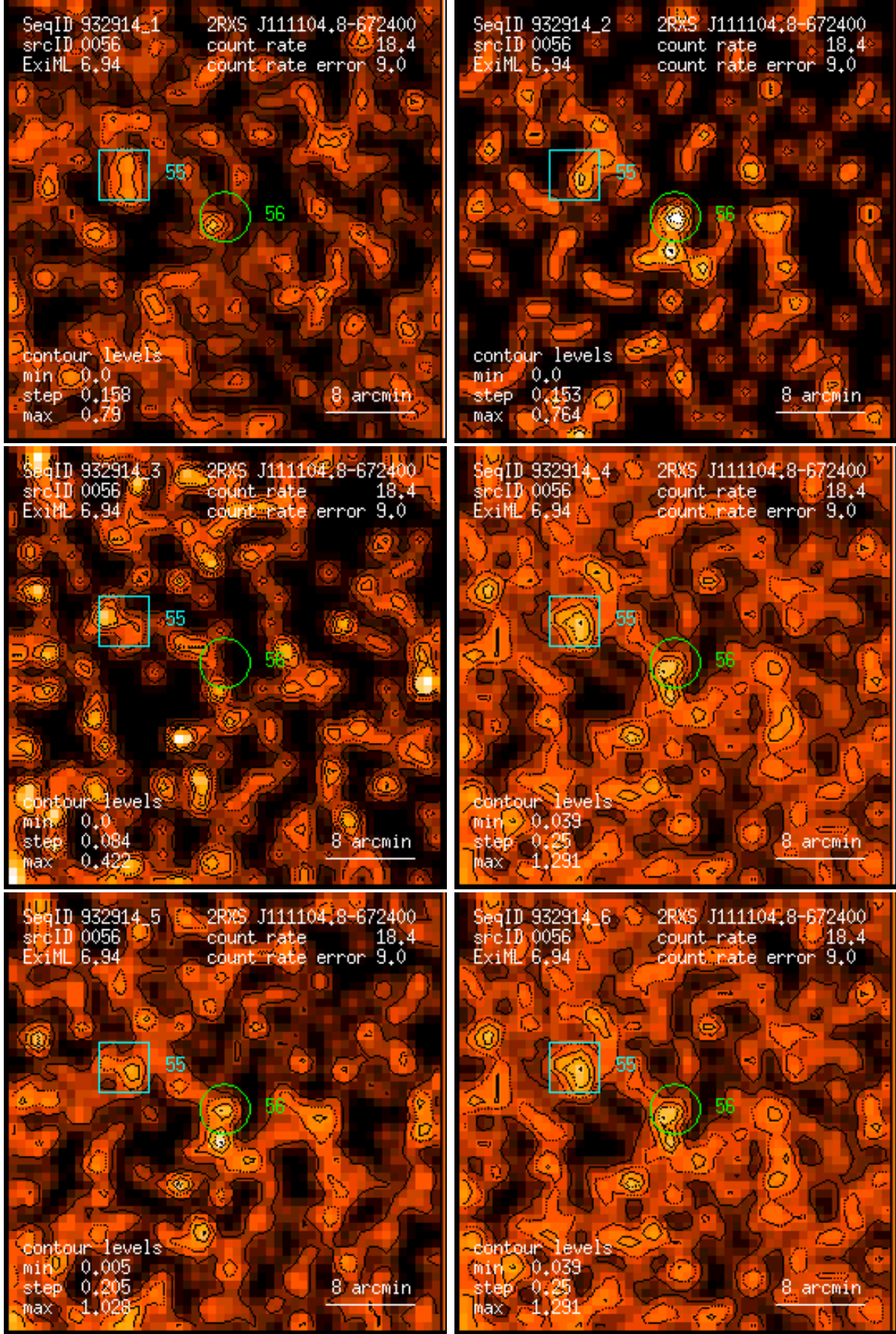
Figure 56: RASS 932914: detection 0056: band rate images, Gaussian filter: (1) PSPC channels 11 – 41, (2) 52 – 90, (3) 91 – 201, (4) 11 – 235, (5) 52 – 201, (6) 11 – 201. Broad band rates in counts/ks. Band rate contour levels in counts/ks/arcmin 2 .
