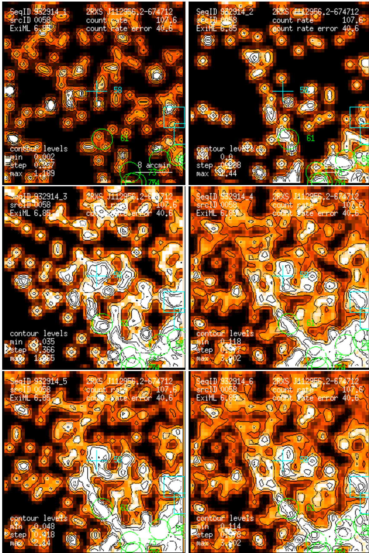
Figure 58: RASS 932914: detection 0058: band rate images, Gaussian filter: (1) PSPC channels 11 – 41, (2) 52 – 90, (3) 91 – 201, (4) 11 – 235, (5) 52 – 201, (6) 11 – 201. Broad band rates in counts/ks. Band rate contour levels in counts/ks/arcmin 2 .
