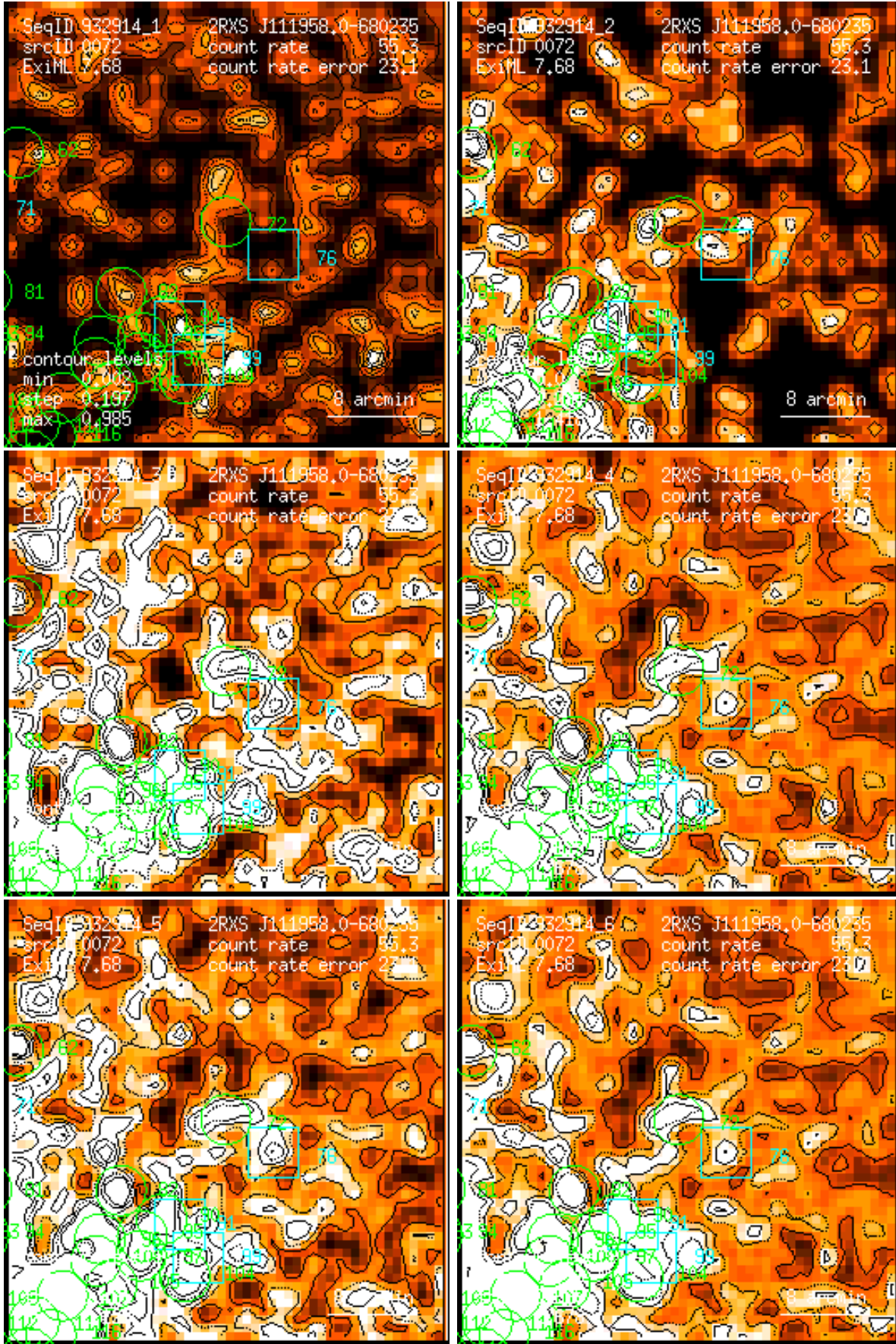
Figure 72: RASS 932914: detection 0072: band rate images, Gaussian filter: (1) PSPC channels 11 – 41, (2) 52 – 90, (3) 91 – 201, (4) 11 – 235, (5) 52 – 201, (6) 11 – 201. Broad band rates in counts/ks. Band rate contour levels in counts/ks/arcmin 2 .
