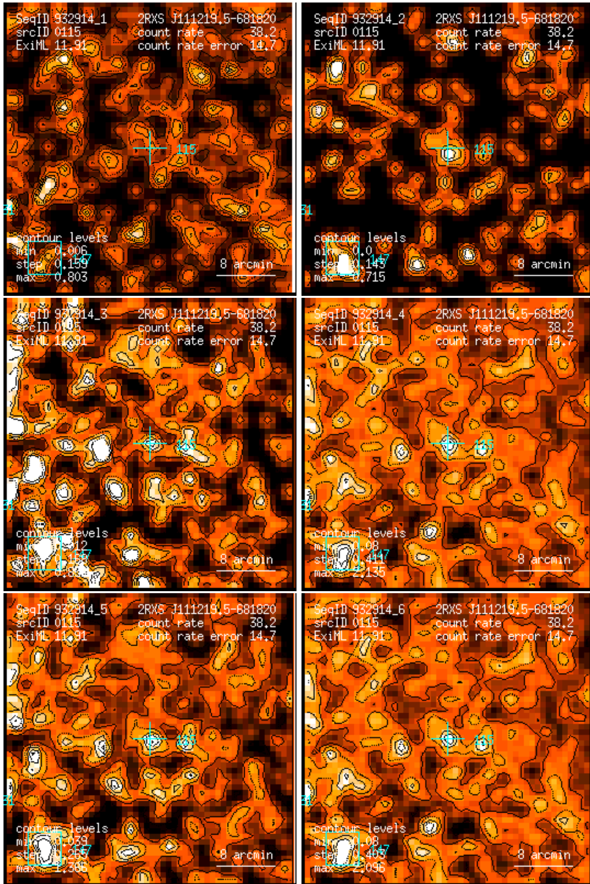
Figure 115: RASS 932914: detection 0115: band rate images, Gaussian filter: (1) PSPC channels 11 – 41, (2) 52 – 90, (3) 91 – 201, (4) 11 – 235, (5) 52 – 201, (6) 11 – 201. Broad band rates in counts/ks. Band rate contour levels in counts/ks/arcmin 2 .
