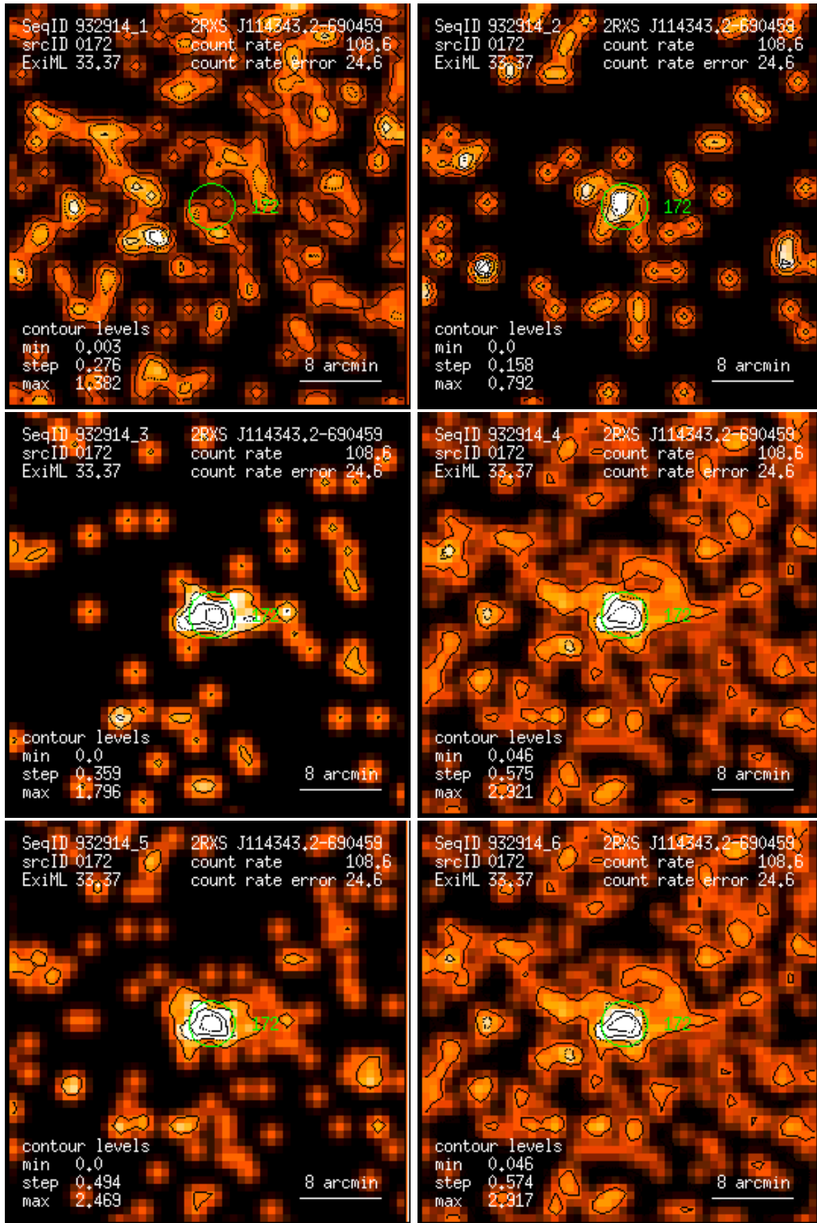
Figure 172: RASS 932914: detection 0172: band rate images, Gaussian filter: (1) PSPC channels 11 – 41, (2) 52 – 90, (3) 91 – 201, (4) 11 – 235, (5) 52 – 201, (6) 11 – 201. Broad band rates in counts/ks. Band rate contour levels in counts/ks/arcmin 2 .
