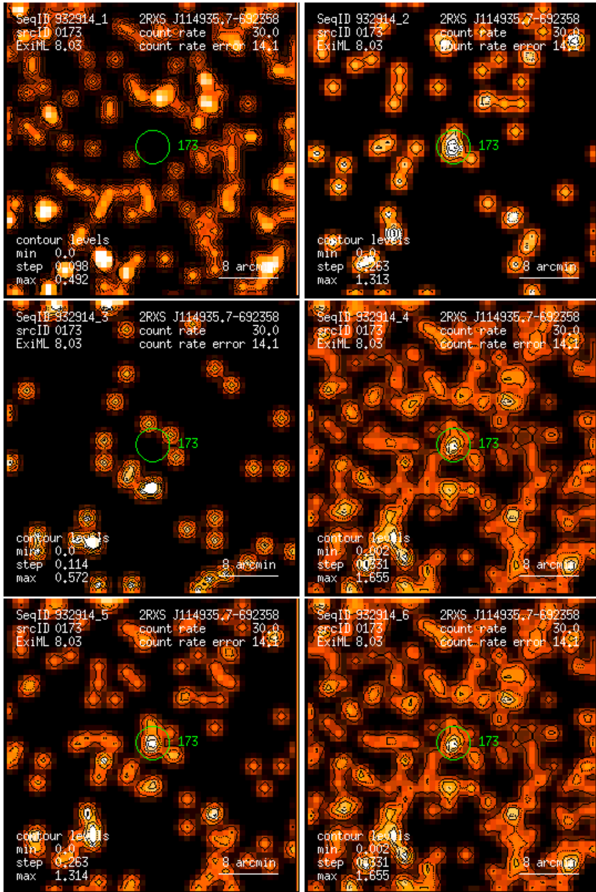
Figure 173: RASS 932914: detection 0173: band rate images, Gaussian filter: (1) PSPC channels 11 – 41, (2) 52 – 90, (3) 91 – 201, (4) 11 – 235, (5) 52 – 201, (6) 11 – 201. Broad band rates in counts/ks. Band rate contour levels in counts/ks/arcmin 2 .
