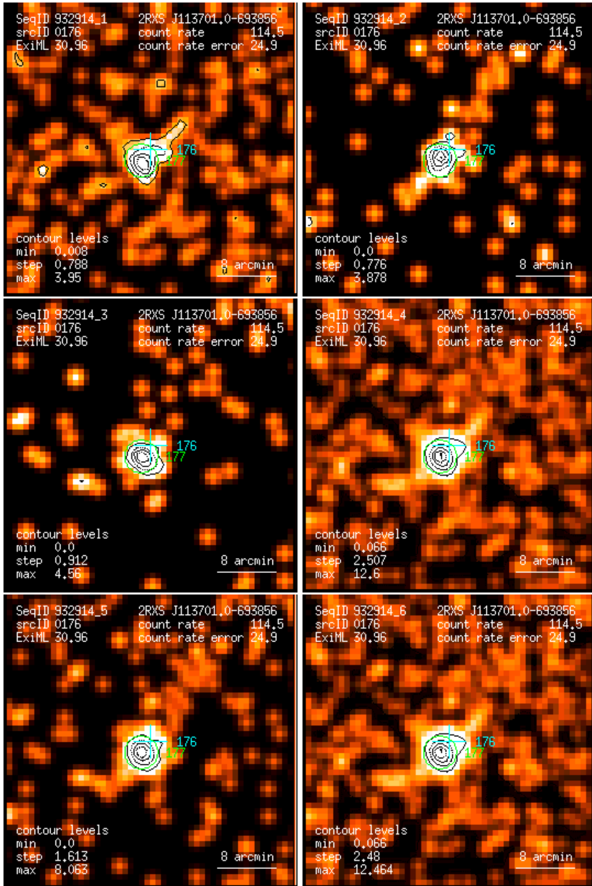
Figure 176: RASS 932914: detection 0176: band rate images, Gaussian filter: (1) PSPC channels 11 – 41, (2) 52 – 90, (3) 91 – 201, (4) 11 – 235, (5) 52 – 201, (6) 11 – 201. Broad band rates in counts/ks. Band rate contour levels in counts/ks/arcmin 2 .
