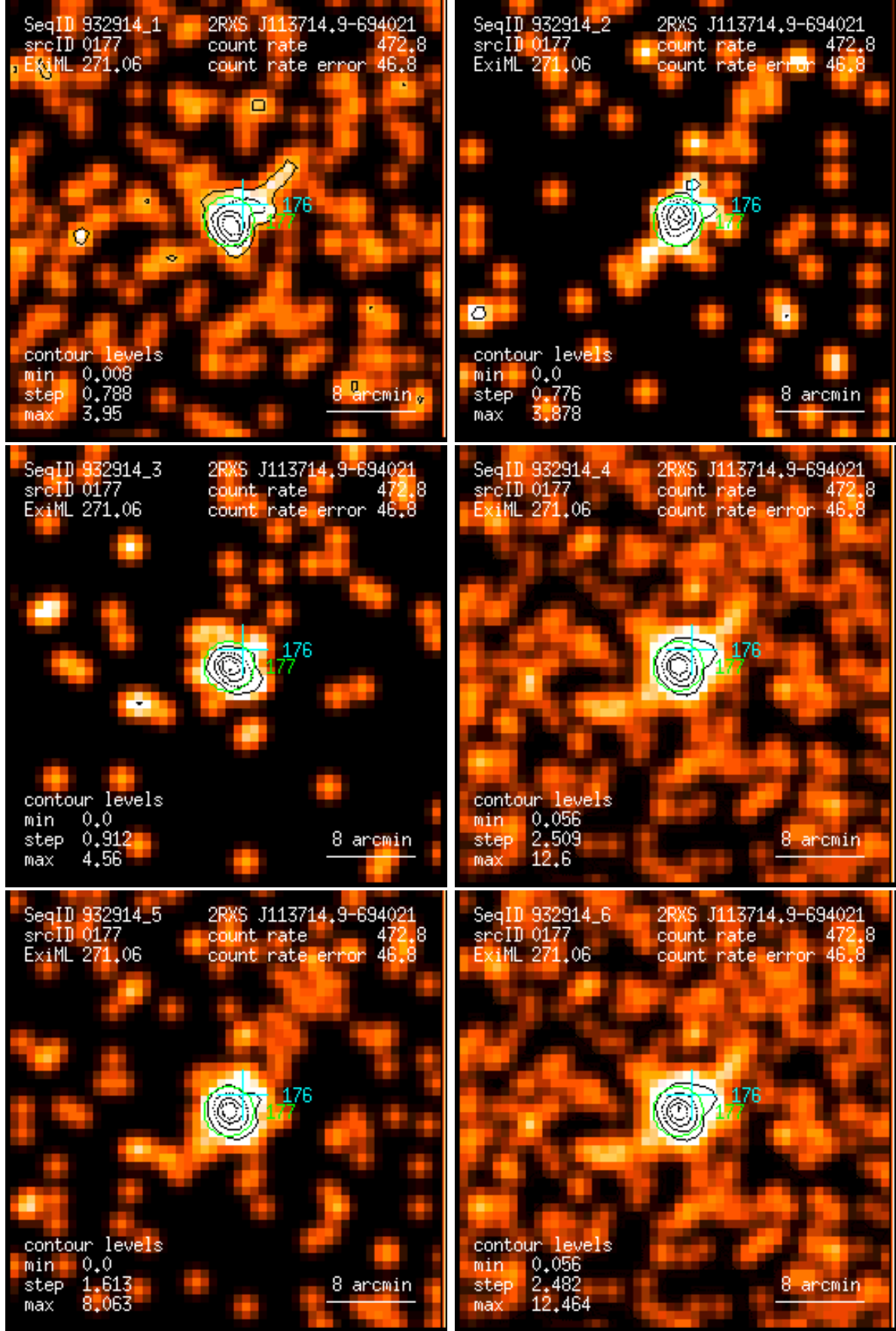
Figure 177: RASS 932914: detection 0177: band rate images, Gaussian filter: (1) PSPC channels 11 – 41, (2) 52 – 90, (3) 91 – 201, (4) 11 – 235, (5) 52 – 201, (6) 11 – 201. Broad band rates in counts/ks. Band rate contour levels in counts/ks/arcmin 2 .
