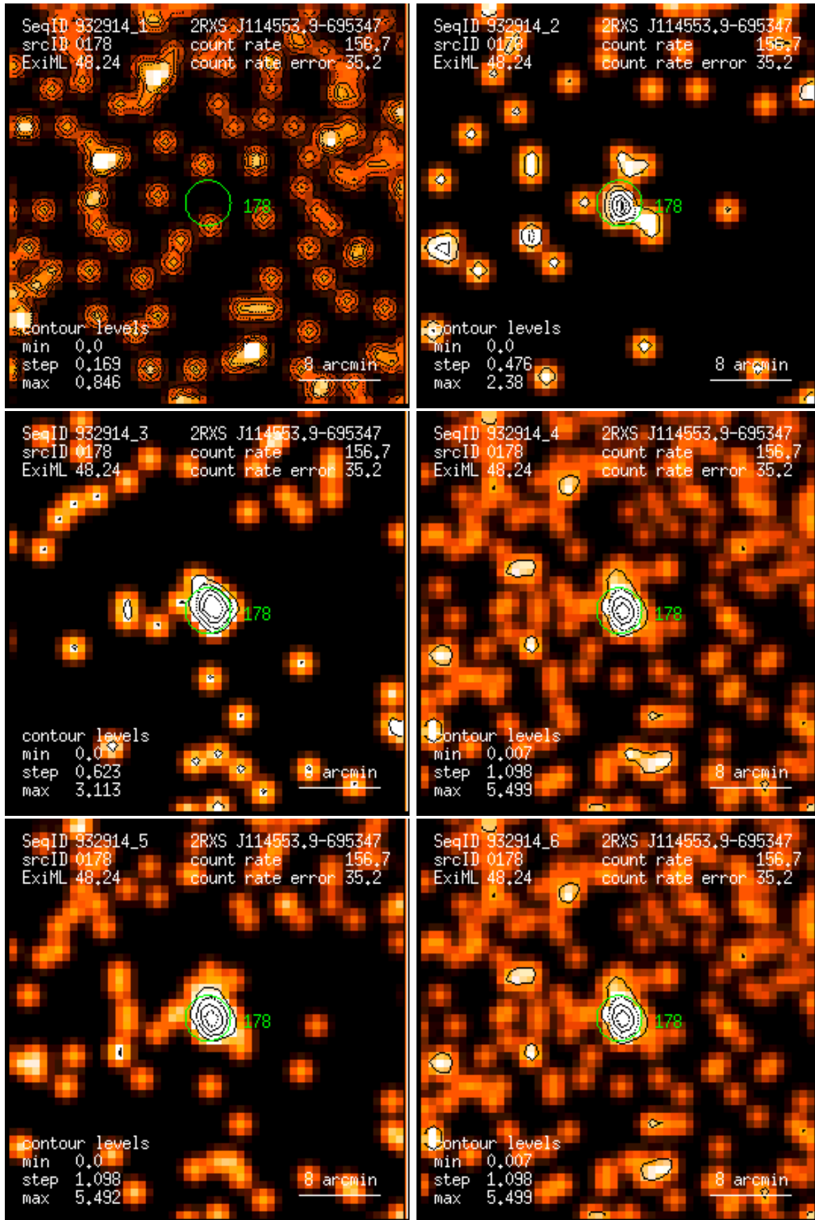
Figure 178: RASS 932914: detection 0178: band rate images, Gaussian filter: (1) PSPC channels 11 – 41, (2) 52 – 90, (3) 91 – 201, (4) 11 – 235, (5) 52 – 201, (6) 11 – 201. Broad band rates in counts/ks. Band rate contour levels in counts/ks/arcmin 2 .
