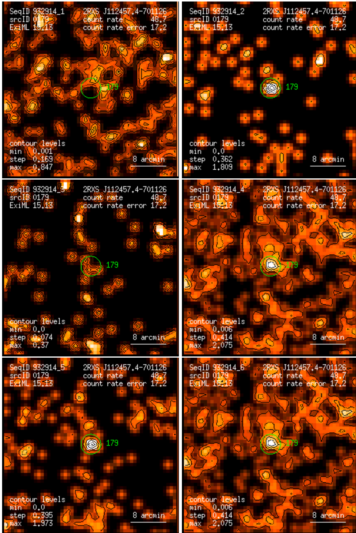
Figure 179: RASS 932914: detection 0179: band rate images, Gaussian filter: (1) PSPC channels 11 – 41, (2) 52 – 90, (3) 91 – 201, (4) 11 – 235, (5) 52 – 201, (6) 11 – 201. Broad band rates in counts/ks. Band rate contour levels in counts/ks/arcmin 2 .
