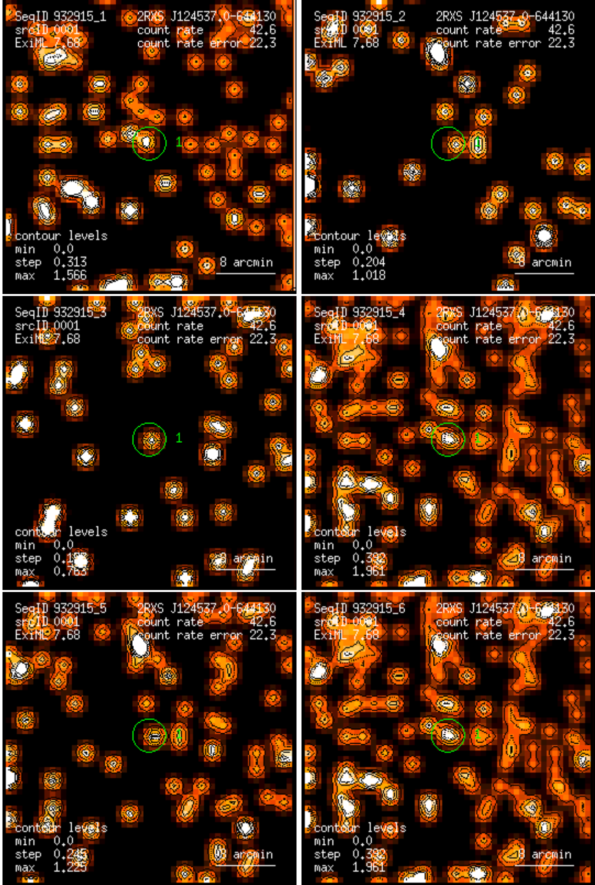
Figure 1: RASS 932915: detection 0001: band rate images, Gaussian filter: (1) PSPC channels 11 – 41, (2) 52 – 90, (3) 91 – 201, (4) 11 – 235, (5) 52 – 201, (6) 11 – 201. Broad band rates in counts/ks. Band rate contour levels in counts/ks/arcmin 2 .
