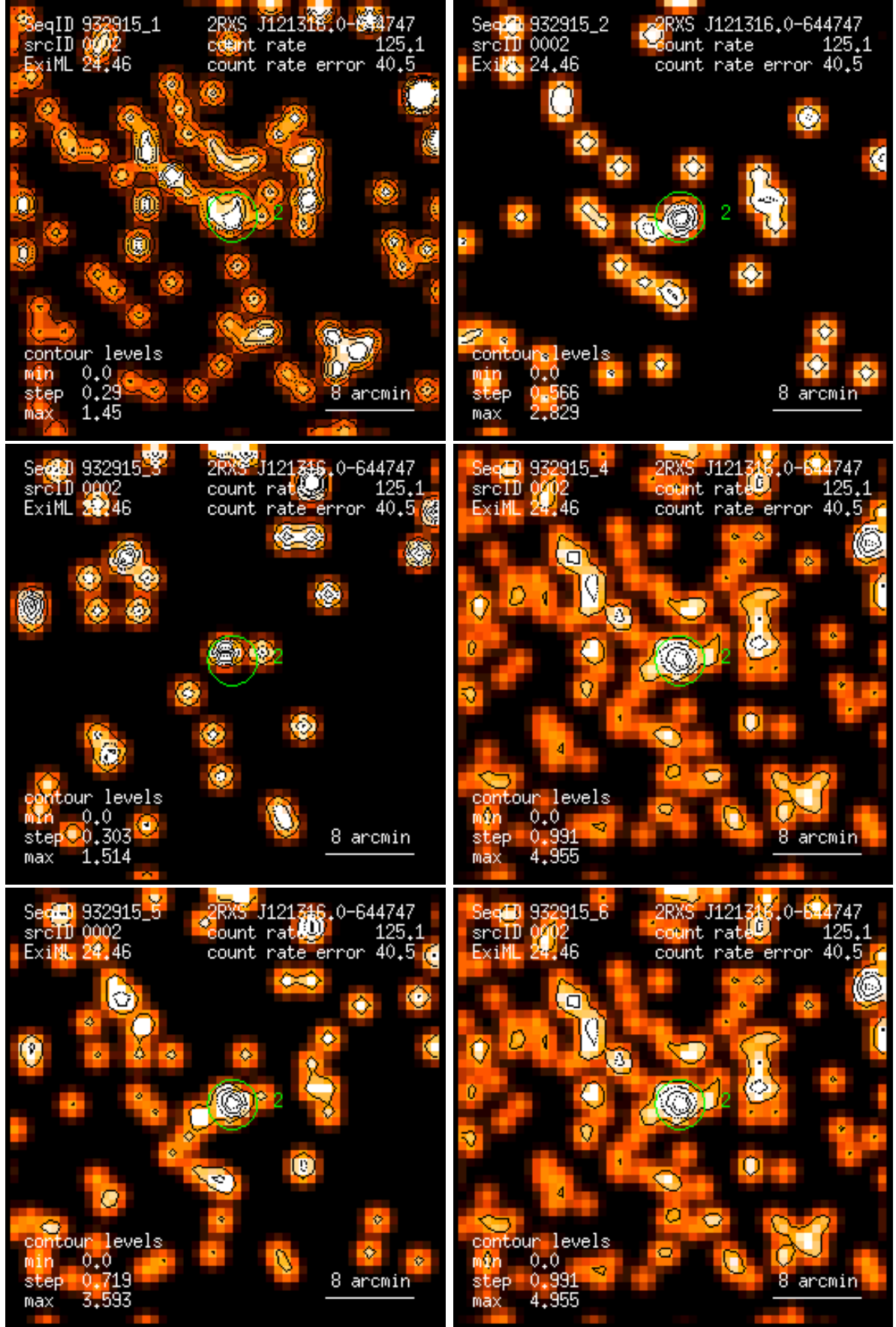
Figure 2: RASS 932915: detection 0002: band rate images, Gaussian filter: (1) PSPC channels 11 – 41, (2) 52 – 90, (3) 91 – 201, (4) 11 – 235, (5) 52 – 201, (6) 11 – 201. Broad band rates in counts/ks. Band rate contour levels in counts/ks/arcmin 2 .
