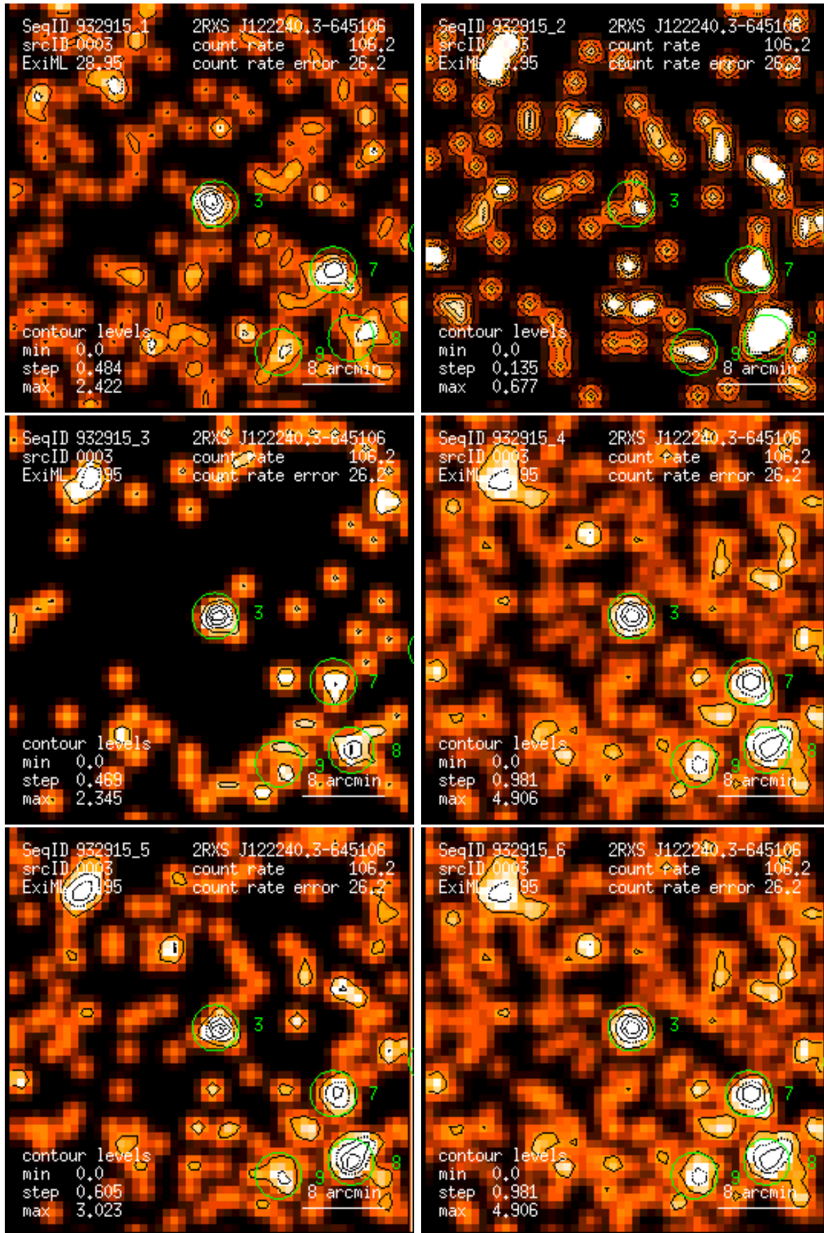
Figure 3: RASS 932915: detection 0003: band rate images, Gaussian filter: (1) PSPC channels 11 – 41, (2) 52 – 90, (3) 91 – 201, (4) 11 – 235, (5) 52 – 201, (6) 11 – 201. Broad band rates in counts/ks. Band rate contour levels in counts/ks/arcmin 2 .
