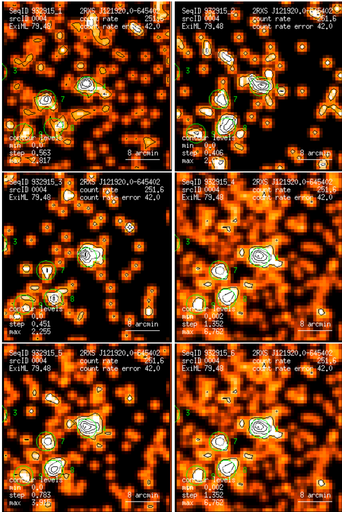
Figure 4: RASS 932915: detection 0004: band rate images, Gaussian filter: (1) PSPC channels 11 – 41, (2) 52 – 90, (3) 91 – 201, (4) 11 – 235, (5) 52 – 201, (6) 11 – 201. Broad band rates in counts/ks. Band rate contour levels in counts/ks/arcmin 2 .
