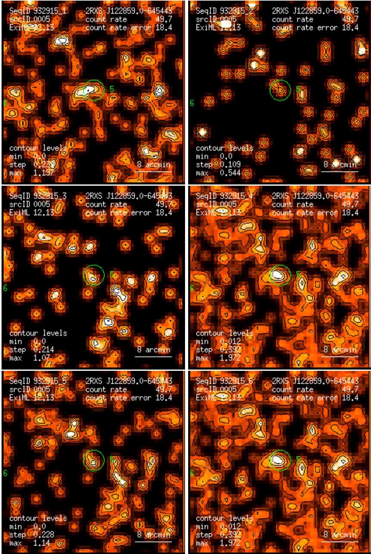
Figure 5: RASS 932915: detection 0005: band rate images, Gaussian filter: (1) PSPC channels 11 – 41, (2) 52 – 90, (3) 91 – 201, (4) 11 – 235, (5) 52 – 201, (6) 11 – 201. Broad band rates in counts/ks. Band rate contour levels in counts/ks/arcmin 2 .
