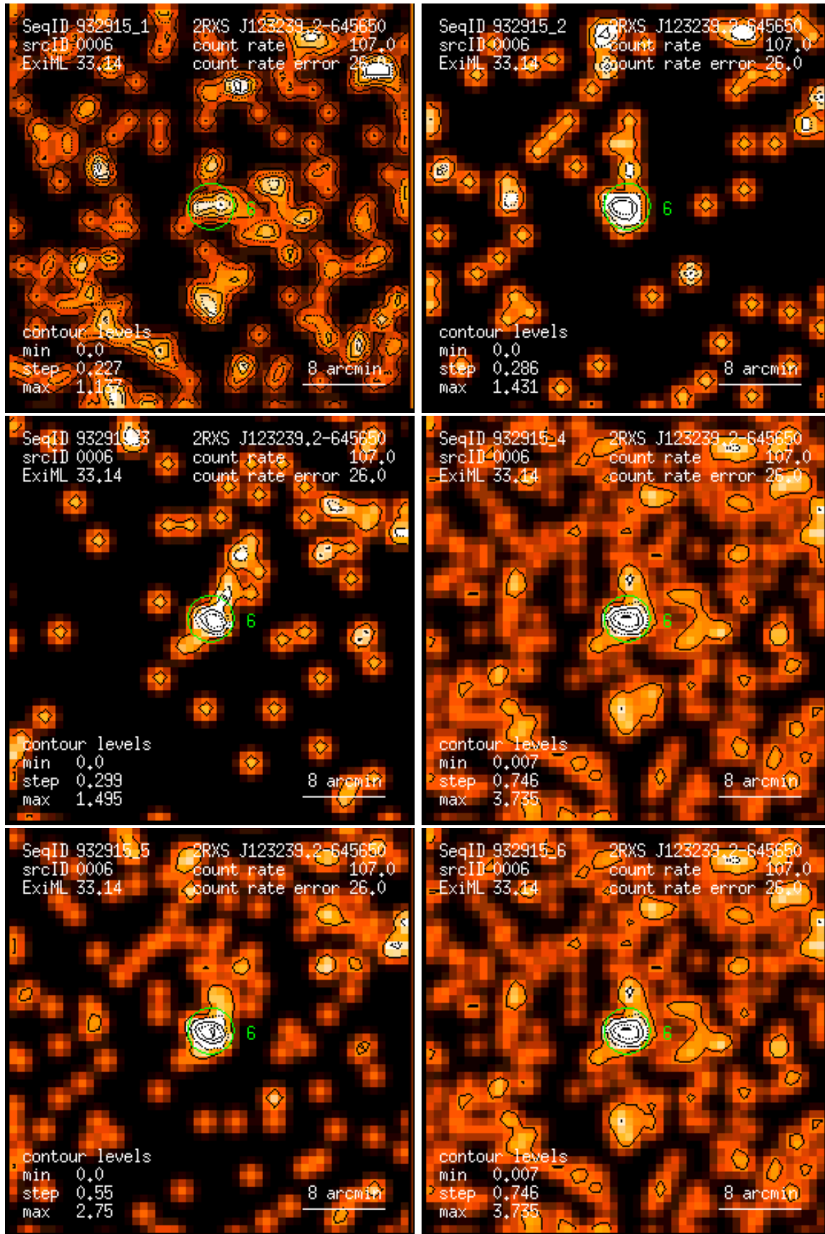
Figure 6: RASS 932915: detection 0006: band rate images, Gaussian filter: (1) PSPC channels 11 – 41, (2) 52 – 90, (3) 91 – 201, (4) 11 – 235, (5) 52 – 201, (6) 11 – 201. Broad band rates in counts/ks. Band rate contour levels in counts/ks/arcmin 2 .
