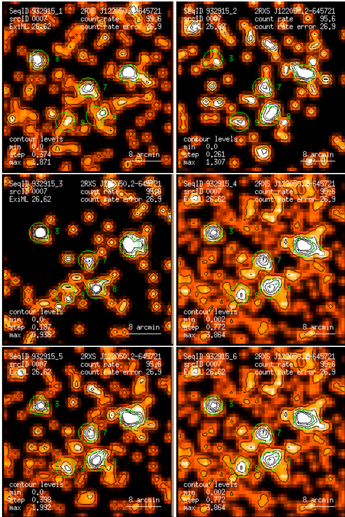
Figure 7: RASS 932915: detection 0007: band rate images, Gaussian filter: (1) PSPC channels 11 – 41, (2) 52 – 90, (3) 91 – 201, (4) 11 – 235, (5) 52 – 201, (6) 11 – 201. Broad band rates in counts/ks. Band rate contour levels in counts/ks/arcmin 2 .
