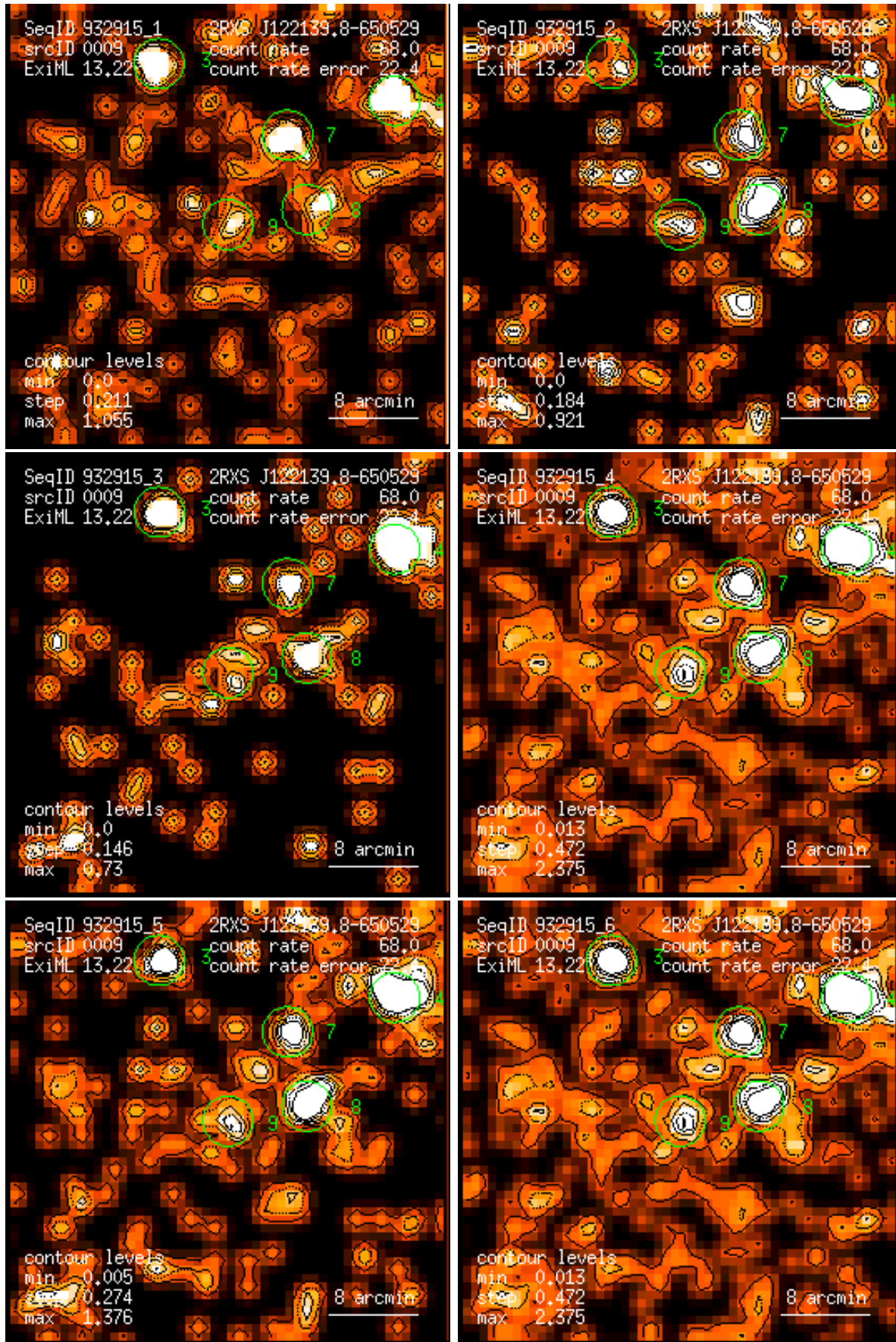
Figure 9: RASS 932915: detection 0009: band rate images, Gaussian filter: (1) PSPC channels 11 – 41, (2) 52 – 90, (3) 91 – 201, (4) 11 – 235, (5) 52 – 201, (6) 11 – 201. Broad band rates in counts/ks. Band rate contour levels in counts/ks/arcmin 2 .
