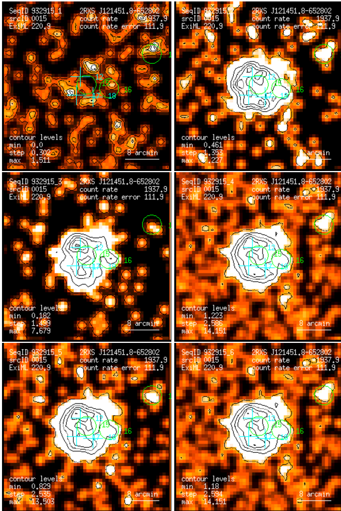
Figure 15: RASS 932915: detection 0015: band rate images, Gaussian filter: (1) PSPC channels 11 – 41, (2) 52 – 90, (3) 91 – 201, (4) 11 – 235, (5) 52 – 201, (6) 11 – 201. Broad band rates in counts/ks. Band rate contour levels in counts/ks/arcmin 2 .
