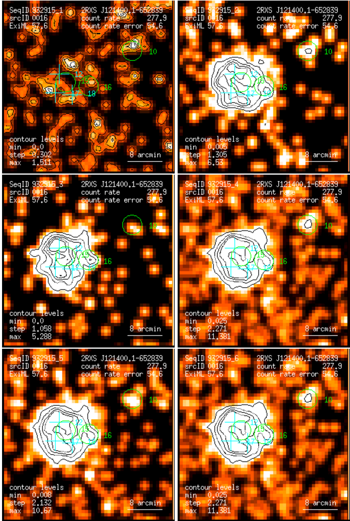
Figure 16: RASS 932915: detection 0016: band rate images, Gaussian filter: (1) PSPC channels 11 – 41, (2) 52 – 90, (3) 91 – 201, (4) 11 – 235, (5) 52 – 201, (6) 11 – 201. Broad band rates in counts/ks. Band rate contour levels in counts/ks/arcmin 2 .
