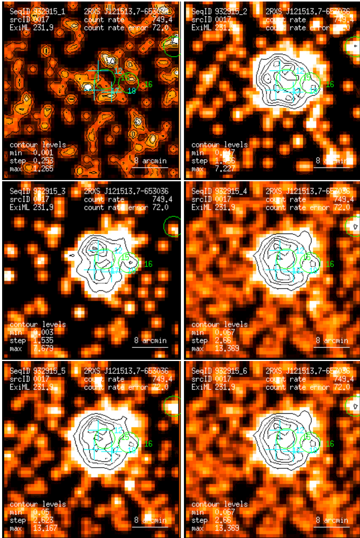
Figure 17: RASS 932915: detection 0017: band rate images, Gaussian filter: (1) PSPC channels 11 – 41, (2) 52 – 90, (3) 91 – 201, (4) 11 – 235, (5) 52 – 201, (6) 11 – 201. Broad band rates in counts/ks. Band rate contour levels in counts/ks/arcmin 2 .
