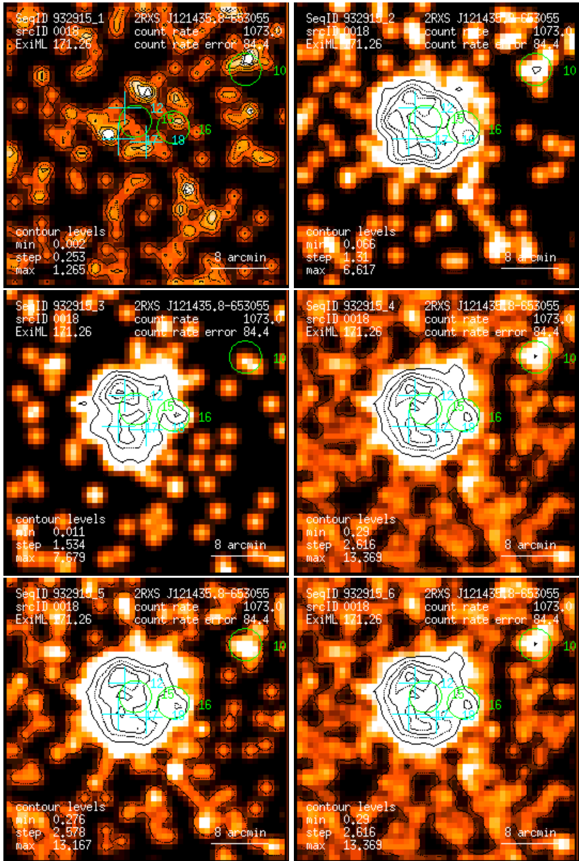
Figure 18: RASS 932915: detection 0018: band rate images, Gaussian filter: (1) PSPC channels 11 – 41, (2) 52 – 90, (3) 91 – 201, (4) 11 – 235, (5) 52 – 201, (6) 11 – 201. Broad band rates in counts/ks. Band rate contour levels in counts/ks/arcmin 2 .
