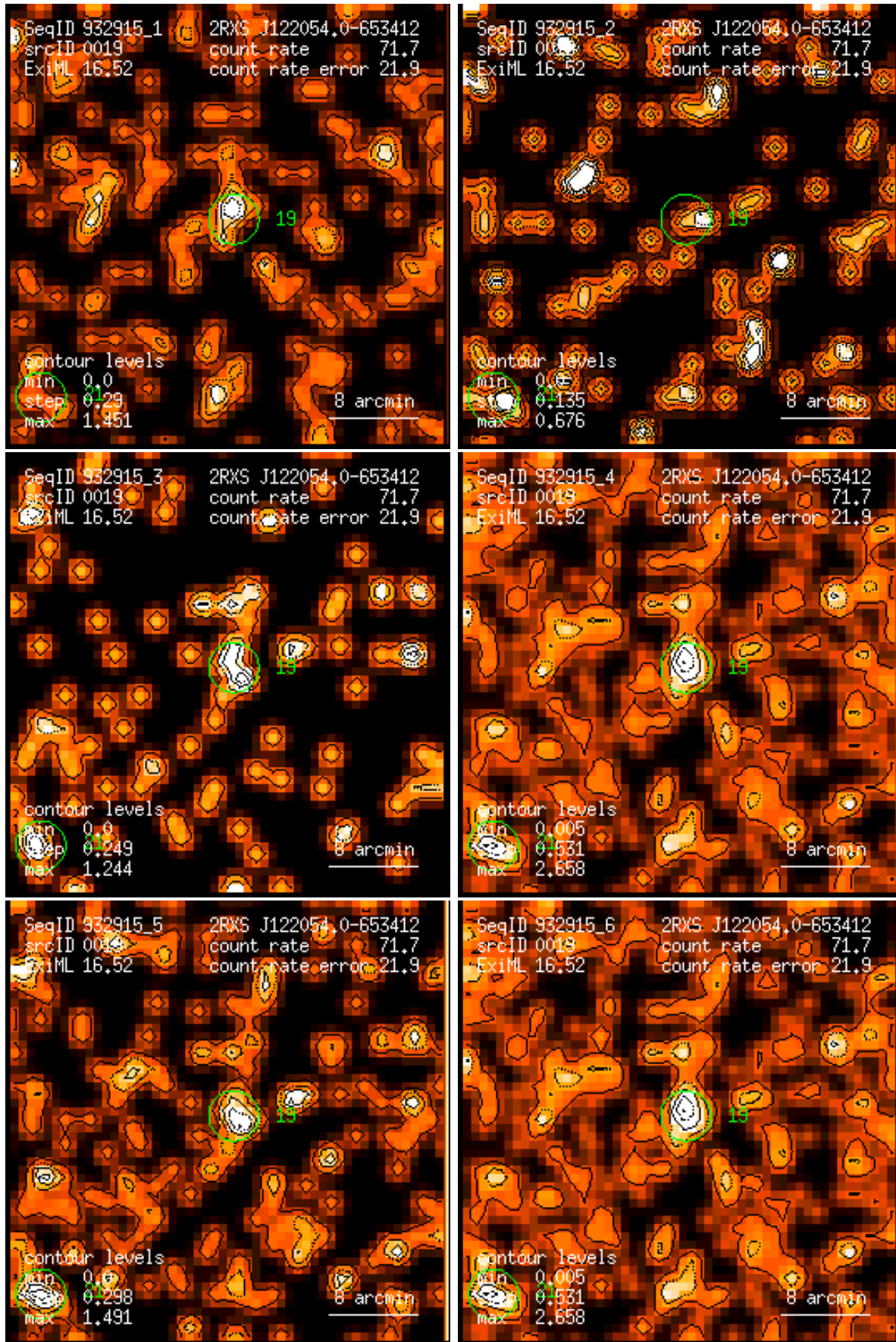
Figure 19: RASS 932915: detection 0019: band rate images, Gaussian filter: (1) PSPC channels 11 – 41, (2) 52 – 90, (3) 91 – 201, (4) 11 – 235, (5) 52 – 201, (6) 11 – 201. Broad band rates in counts/ks. Band rate contour levels in counts/ks/arcmin 2 .
