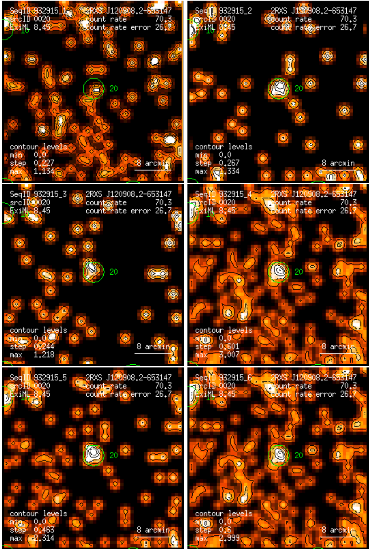
Figure 20: RASS 932915: detection 0020: band rate images, Gaussian filter: (1) PSPC channels 11 – 41, (2) 52 – 90, (3) 91 – 201, (4) 11 – 235, (5) 52 – 201, (6) 11 – 201. Broad band rates in counts/ks. Band rate contour levels in counts/ks/arcmin 2 .
