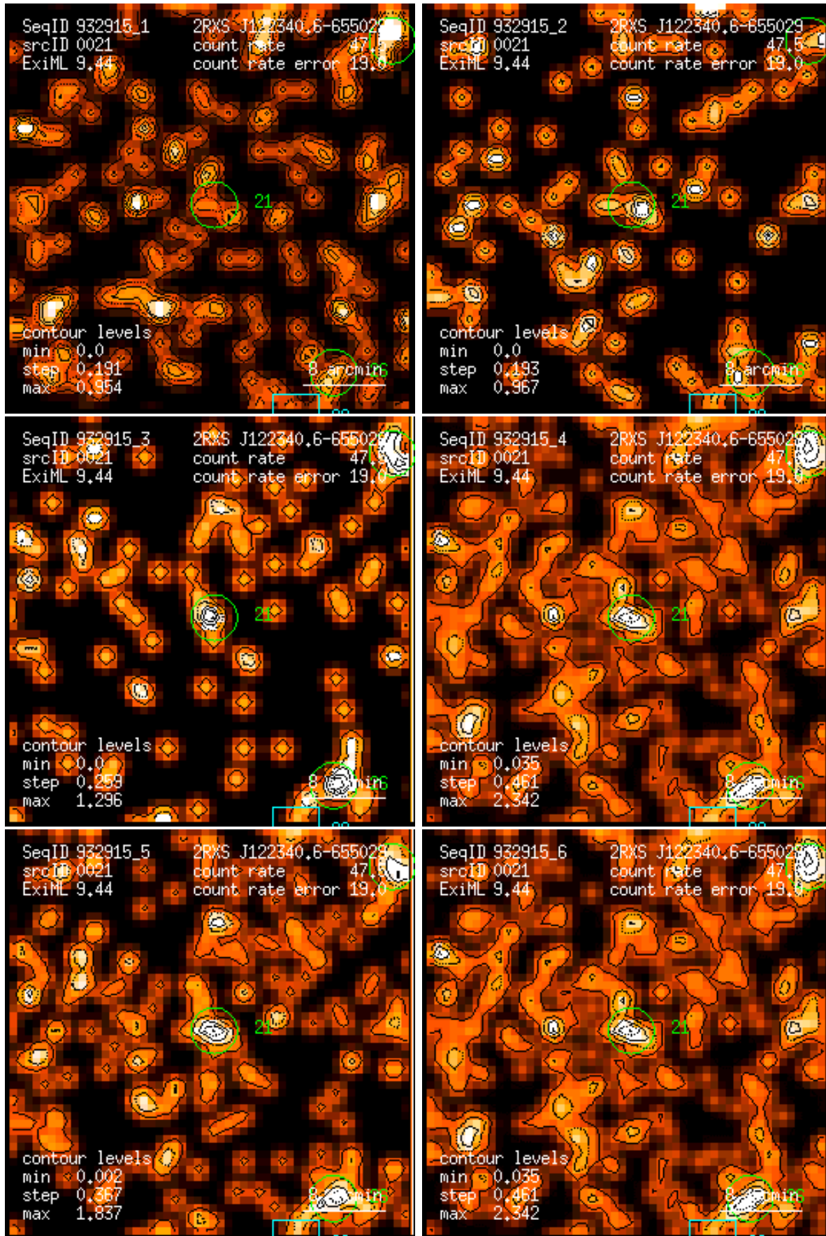
Figure 21: RASS 932915: detection 0021: band rate images, Gaussian filter: (1) PSPC channels 11 – 41, (2) 52 – 90, (3) 91 – 201, (4) 11 – 235, (5) 52 – 201, (6) 11 – 201. Broad band rates in counts/ks. Band rate contour levels in counts/ks/arcmin 2 .
