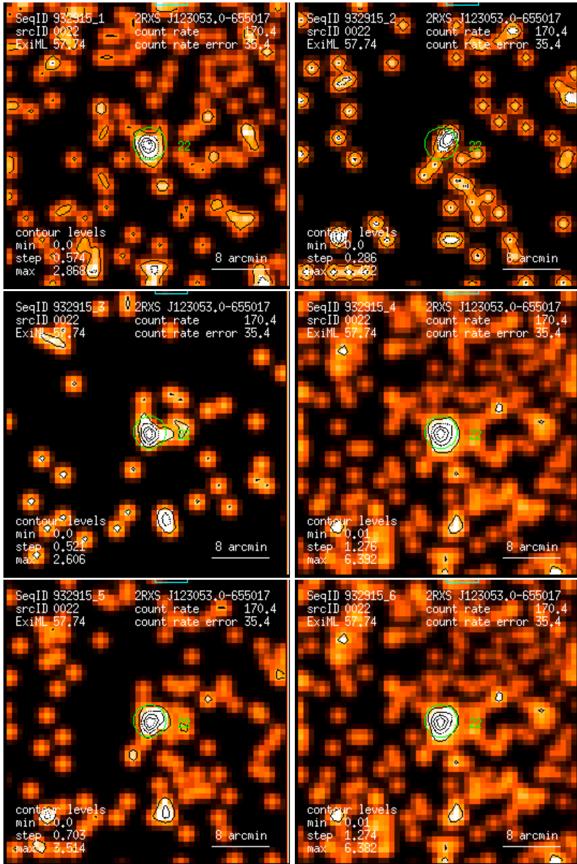
Figure 22: RASS 932915: detection 0022: band rate images, Gaussian filter: (1) PSPC channels 11 – 41, (2) 52 – 90, (3) 91 – 201, (4) 11 – 235, (5) 52 – 201, (6) 11 – 201. Broad band rates in counts/ks. Band rate contour levels in counts/ks/arcmin 2 .
