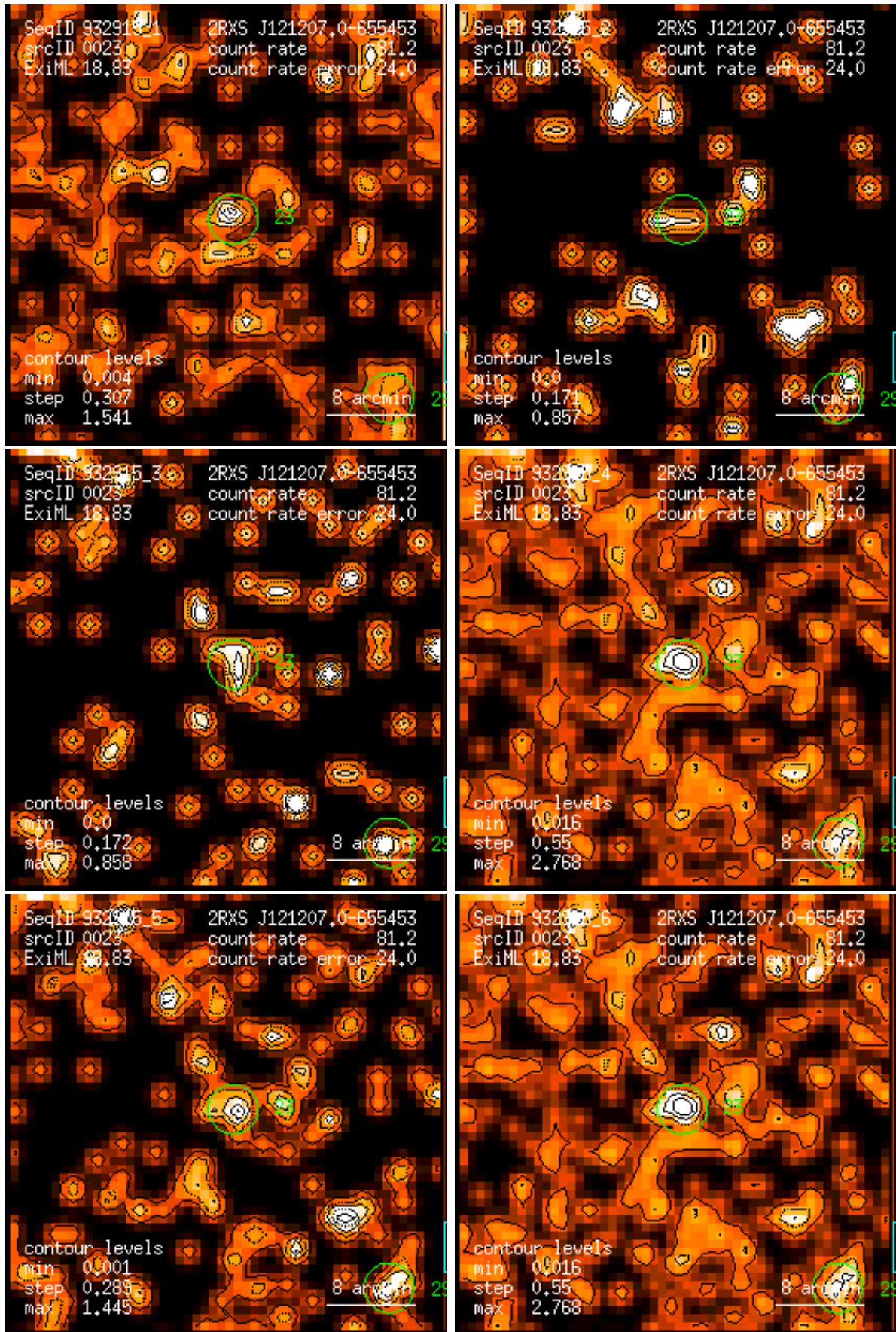
Figure 23: RASS 932915: detection 0023: band rate images, Gaussian filter: (1) PSPC channels 11 – 41, (2) 52 – 90, (3) 91 – 201, (4) 11 – 235, (5) 52 – 201, (6) 11 – 201. Broad band rates in counts/ks. Band rate contour levels in counts/ks/arcmin 2 .
