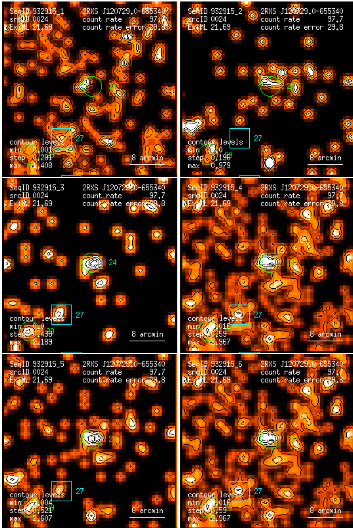
Figure 24: RASS 932915: detection 0024: band rate images, Gaussian filter: (1) PSPC channels 11 – 41, (2) 52 – 90, (3) 91 – 201, (4) 11 – 235, (5) 52 – 201, (6) 11 – 201. Broad band rates in counts/ks. Band rate contour levels in counts/ks/arcmin 2 .
