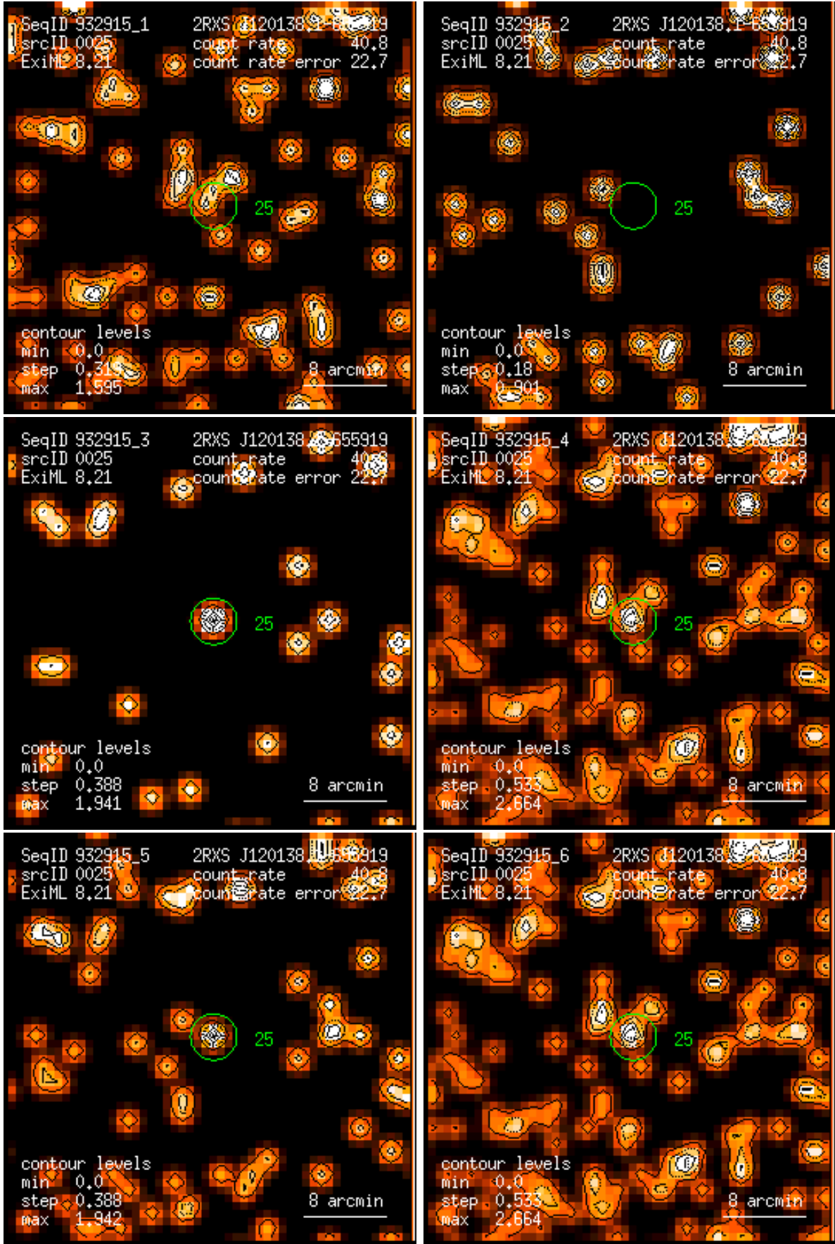
Figure 25: RASS 932915: detection 0025: band rate images, Gaussian filter: (1) PSPC channels 11 – 41, (2) 52 – 90, (3) 91 – 201, (4) 11 – 235, (5) 52 – 201, (6) 11 – 201. Broad band rates in counts/ks. Band rate contour levels in counts/ks/arcmin 2 .
