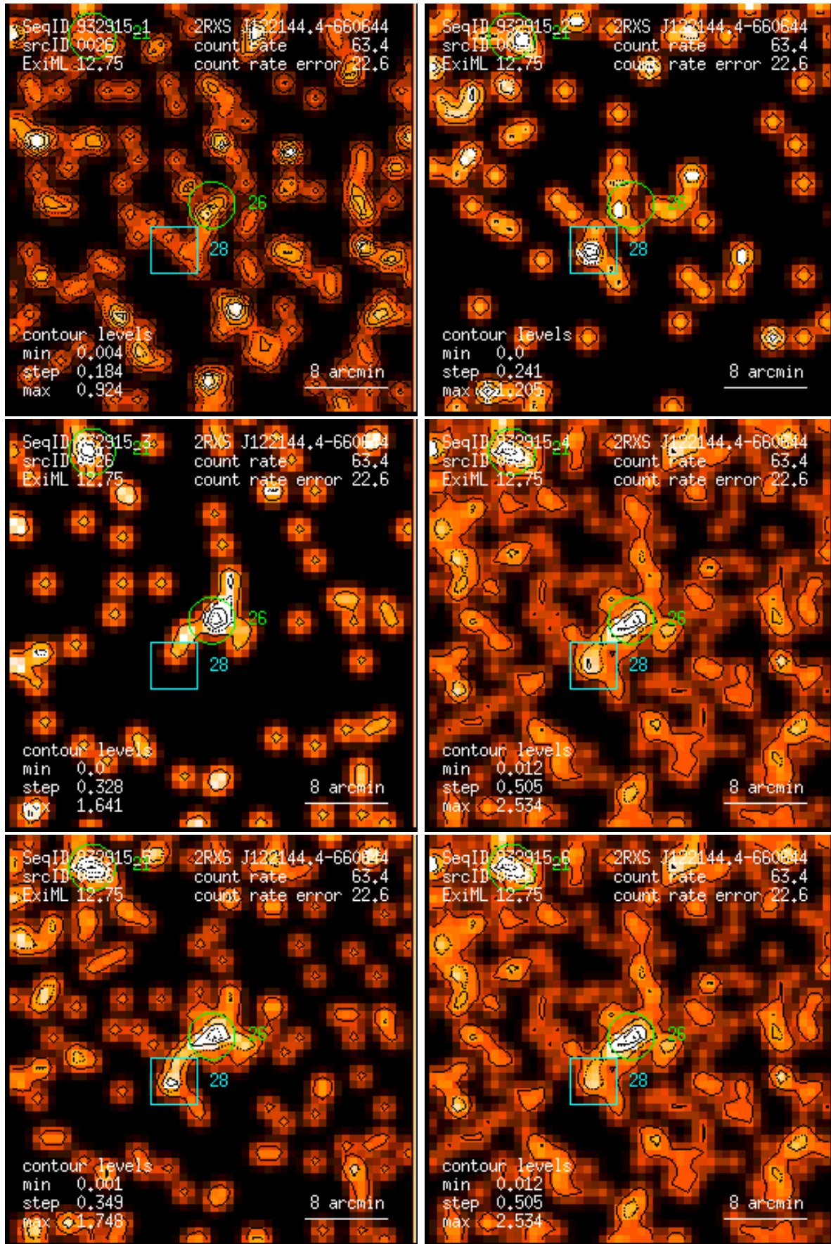
Figure 26: RASS 932915: detection 0026: band rate images, Gaussian filter: (1) PSPC channels 11 – 41, (2) 52 – 90, (3) 91 – 201, (4) 11 – 235, (5) 52 – 201, (6) 11 – 201. Broad band rates in counts/ks. Band rate contour levels in counts/ks/arcmin 2 .
