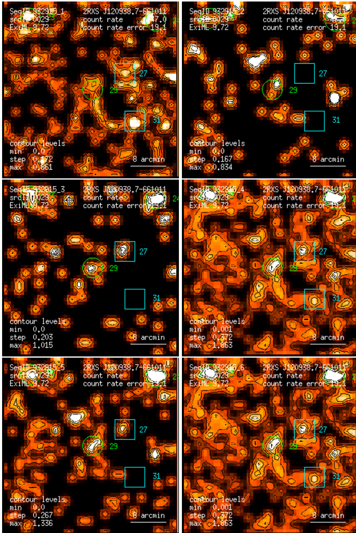
Figure 29: RASS 932915: detection 0029: band rate images, Gaussian filter: (1) PSPC channels 11 – 41, (2) 52 – 90, (3) 91 – 201, (4) 11 – 235, (5) 52 – 201, (6) 11 – 201. Broad band rates in counts/ks. Band rate contour levels in counts/ks/arcmin 2 .
