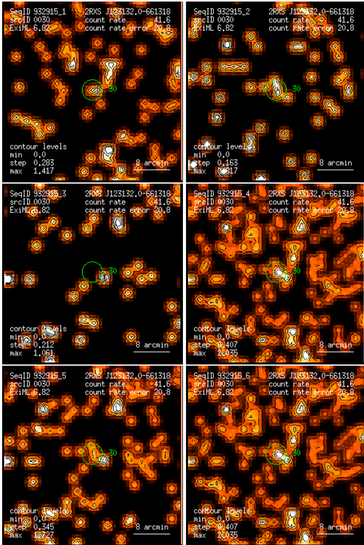
Figure 30: RASS 932915: detection 0030: band rate images, Gaussian filter: (1) PSPC channels 11 – 41, (2) 52 – 90, (3) 91 – 201, (4) 11 – 235, (5) 52 – 201, (6) 11 – 201. Broad band rates in counts/ks. Band rate contour levels in counts/ks/arcmin 2 .
