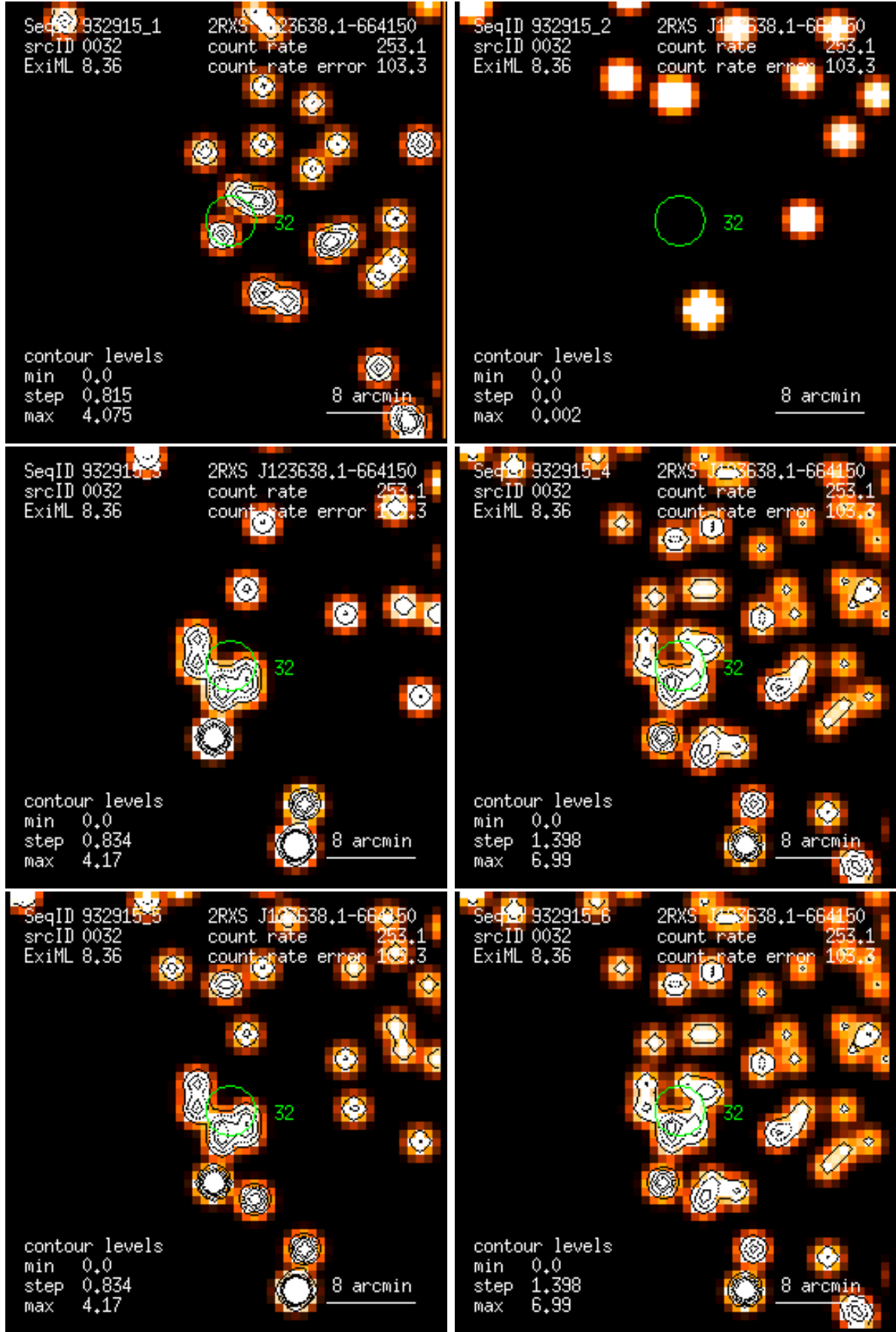
Figure 32: RASS 932915: detection 0032: band rate images, Gaussian filter: (1) PSPC channels 11 – 41, (2) 52 – 90, (3) 91 – 201, (4) 11 – 235, (5) 52 – 201, (6) 11 – 201. Broad band rates in counts/ks. Band rate contour levels in counts/ks/arcmin 2 .
