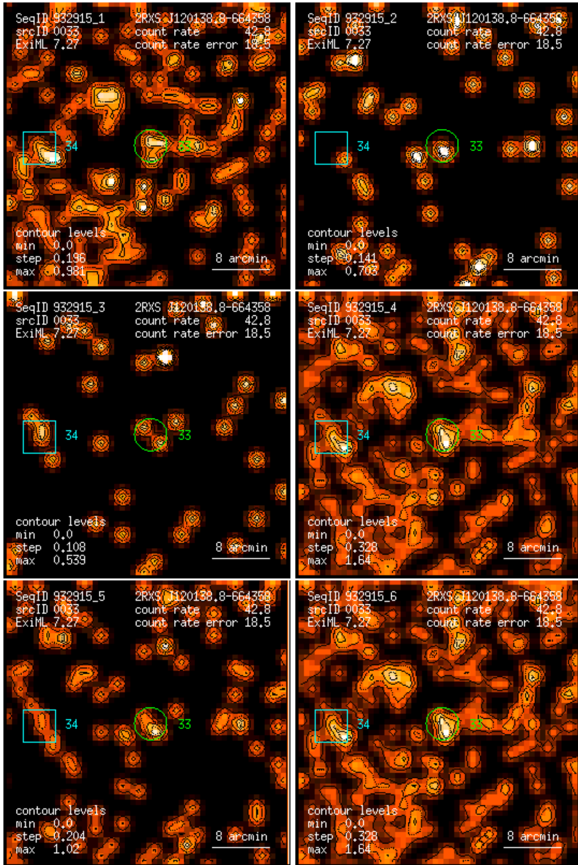
Figure 33: RASS 932915: detection 0033: band rate images, Gaussian filter: (1) PSPC channels 11 – 41, (2) 52 – 90, (3) 91 – 201, (4) 11 – 235, (5) 52 – 201, (6) 11 – 201. Broad band rates in counts/ks. Band rate contour levels in counts/ks/arcmin 2 .
