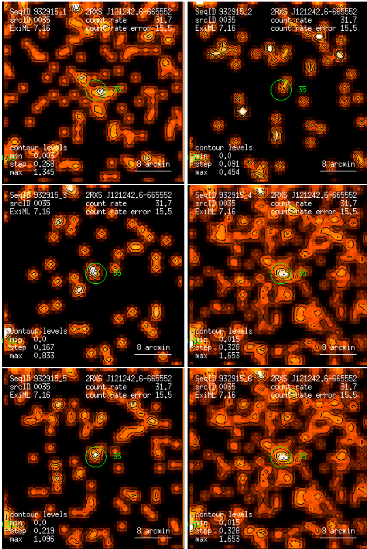
Figure 35: RASS 932915: detection 0035: band rate images, Gaussian filter: (1) PSPC channels 11 – 41, (2) 52 – 90, (3) 91 – 201, (4) 11 – 235, (5) 52 – 201, (6) 11 – 201. Broad band rates in counts/ks. Band rate contour levels in counts/ks/arcmin 2 .
