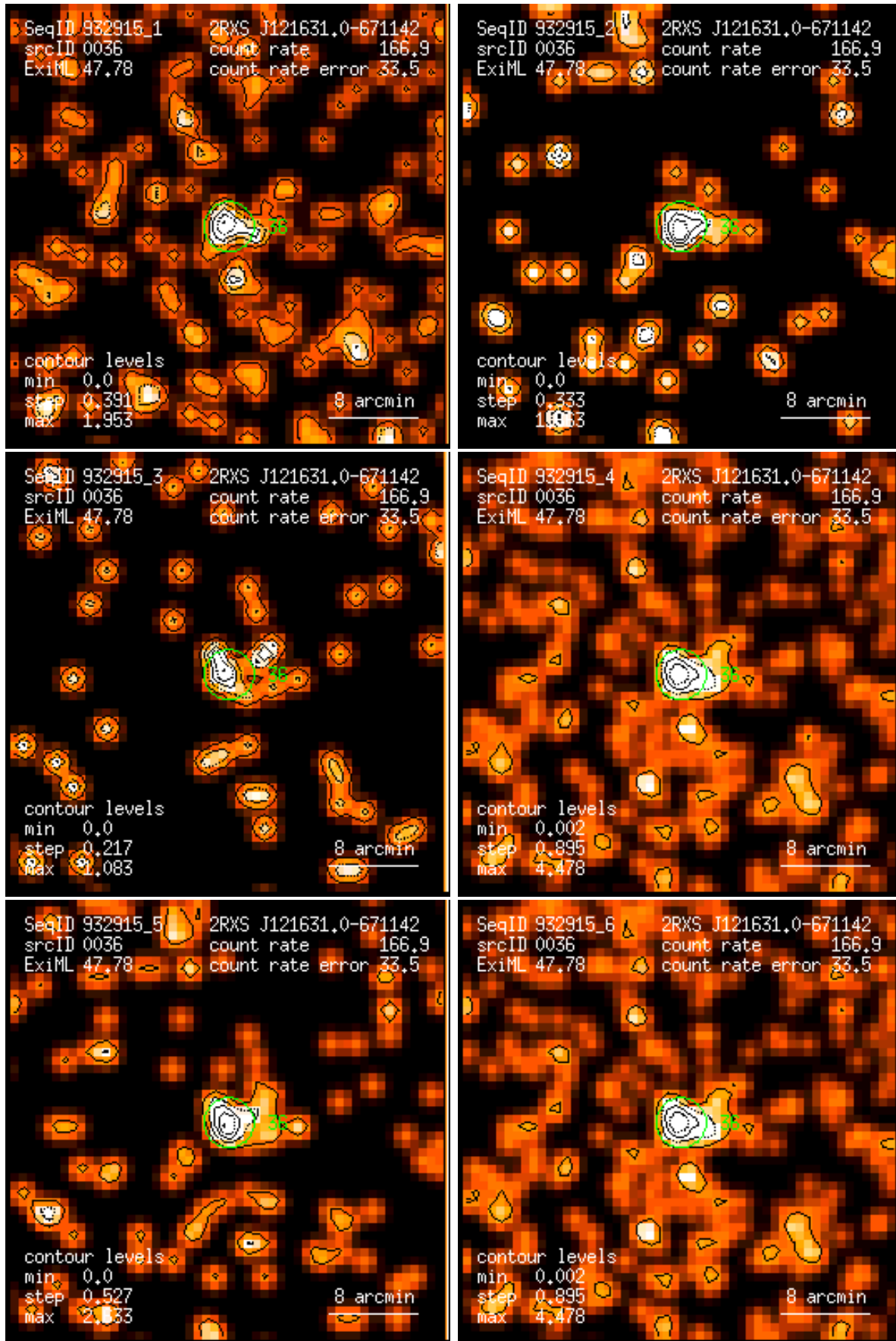
Figure 36: RASS 932915: detection 0036: band rate images, Gaussian filter: (1) PSPC channels 11 – 41, (2) 52 – 90, (3) 91 – 201, (4) 11 – 235, (5) 52 – 201, (6) 11 – 201. Broad band rates in counts/ks. Band rate contour levels in counts/ks/arcmin 2 .
