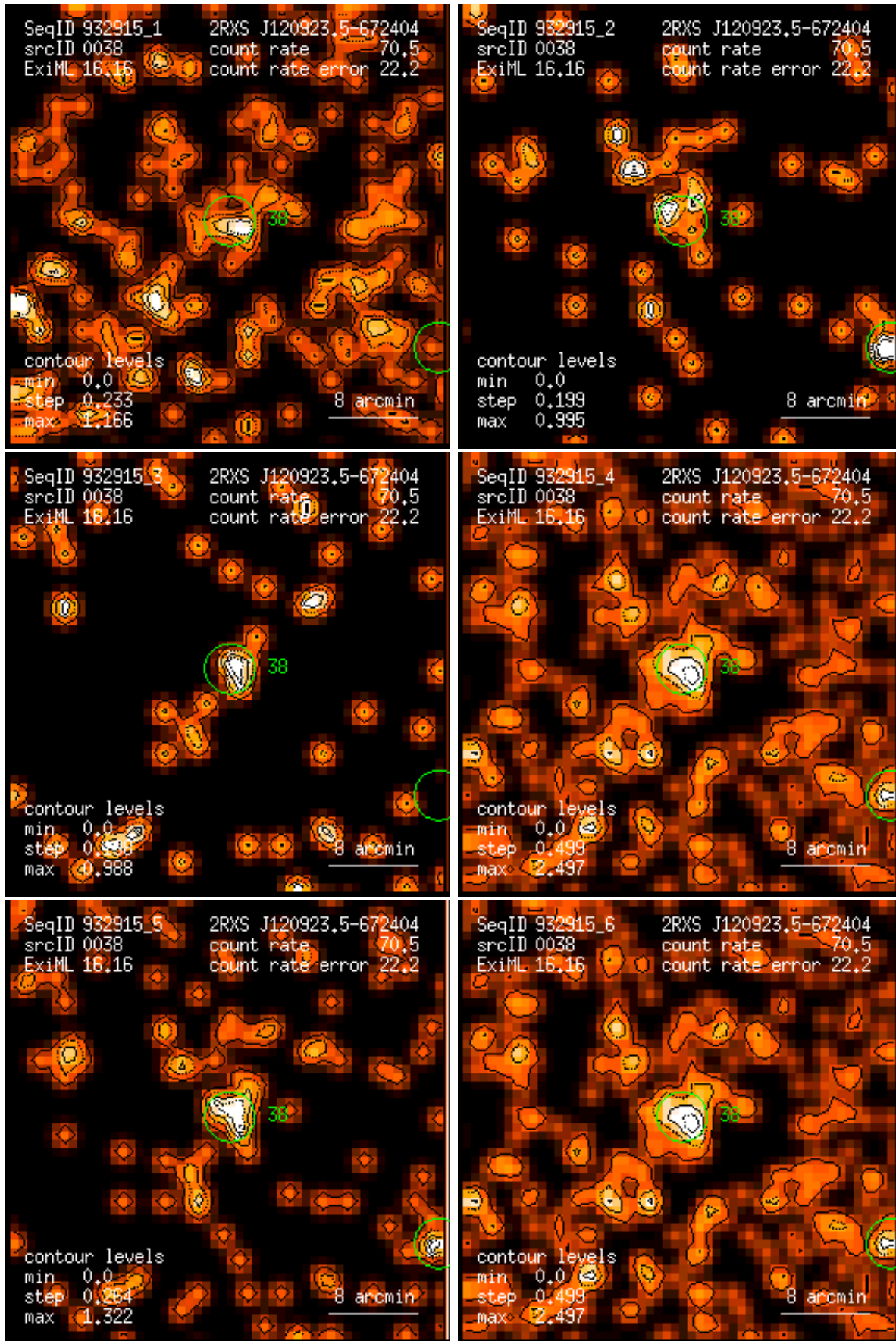
Figure 38: RASS 932915: detection 0038: band rate images, Gaussian filter: (1) PSPC channels 11 – 41, (2) 52 – 90, (3) 91 – 201, (4) 11 – 235, (5) 52 – 201, (6) 11 – 201. Broad band rates in counts/ks. Band rate contour levels in counts/ks/arcmin 2 .
