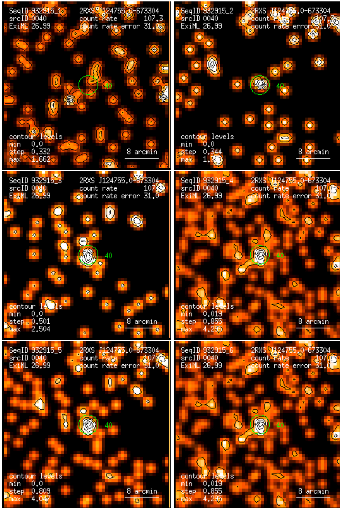
Figure 40: RASS 932915: detection 0040: band rate images, Gaussian filter: (1) PSPC channels 11 – 41, (2) 52 – 90, (3) 91 – 201, (4) 11 – 235, (5) 52 – 201, (6) 11 – 201. Broad band rates in counts/ks. Band rate contour levels in counts/ks/arcmin 2 .
