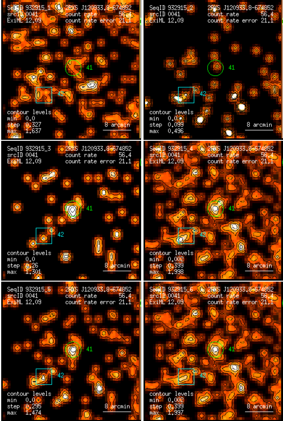
Figure 41: RASS 932915: detection 0041: band rate images, Gaussian filter: (1) PSPC channels 11 – 41, (2) 52 – 90, (3) 91 – 201, (4) 11 – 235, (5) 52 – 201, (6) 11 – 201. Broad band rates in counts/ks. Band rate contour levels in counts/ks/arcmin 2 .
