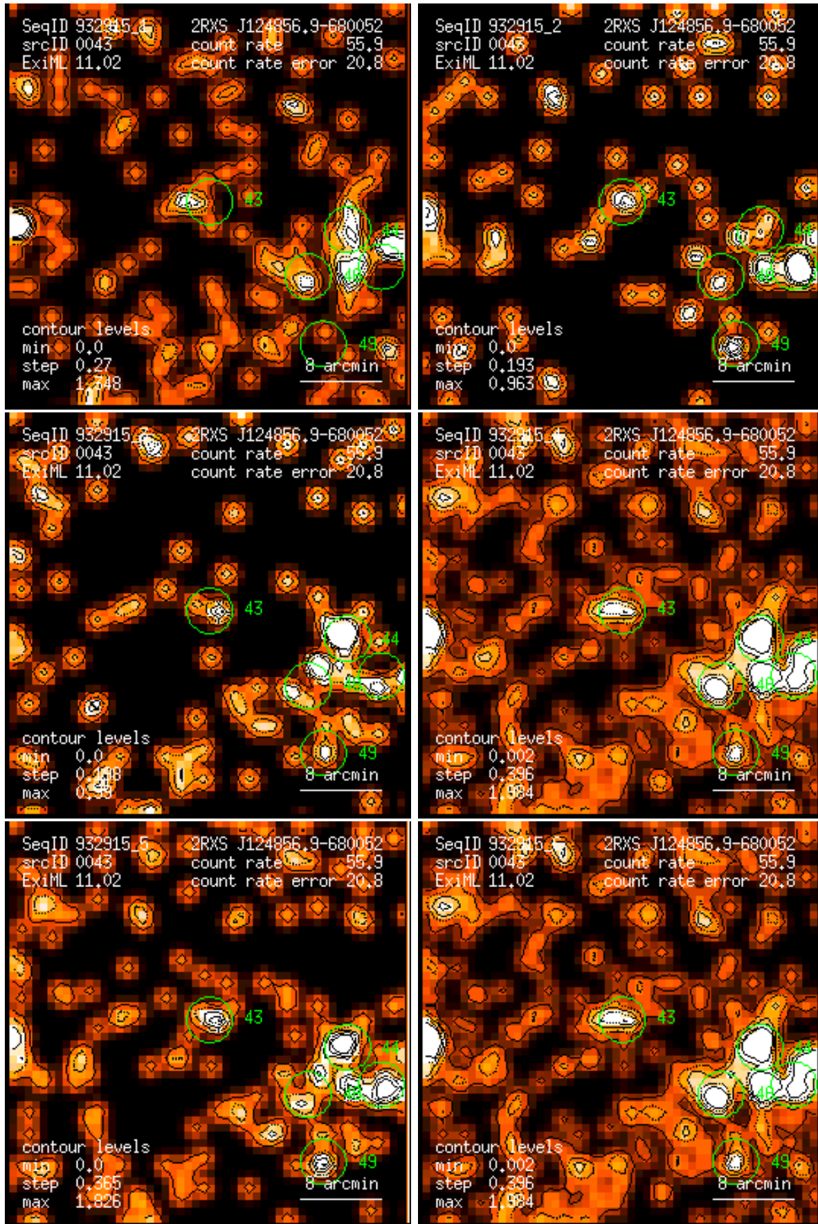
Figure 43: RASS 932915: detection 0043: band rate images, Gaussian filter: (1) PSPC channels 11 – 41, (2) 52 – 90, (3) 91 – 201, (4) 11 – 235, (5) 52 – 201, (6) 11 – 201. Broad band rates in counts/ks. Band rate contour levels in counts/ks/arcmin 2 .
