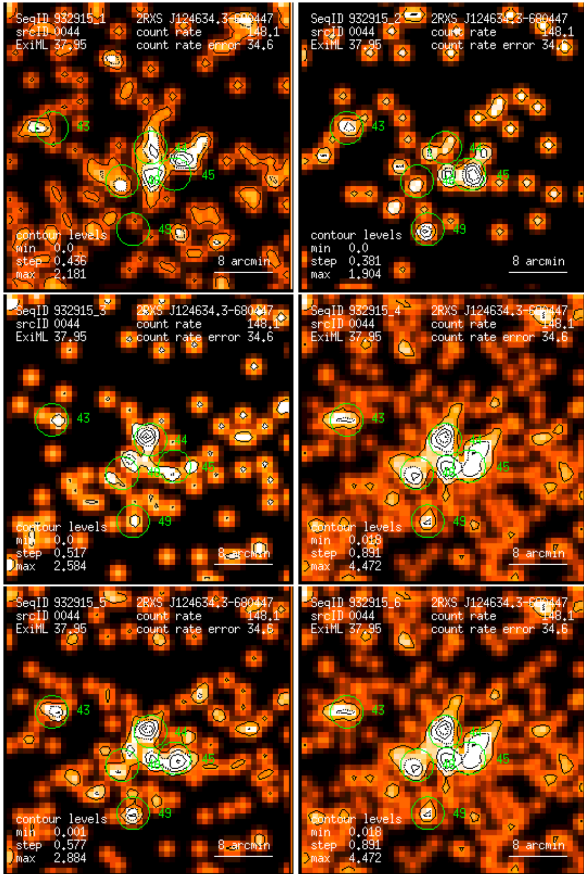
Figure 44: RASS 932915: detection 0044: band rate images, Gaussian filter: (1) PSPC channels 11 – 41, (2) 52 – 90, (3) 91 – 201, (4) 11 – 235, (5) 52 – 201, (6) 11 – 201. Broad band rates in counts/ks. Band rate contour levels in counts/ks/arcmin 2 .
